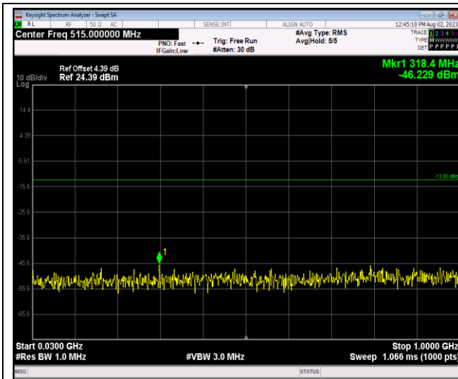
Band4-1.4MHz-QPSK-19957-1RB#0-Range1:30~1000MHz
