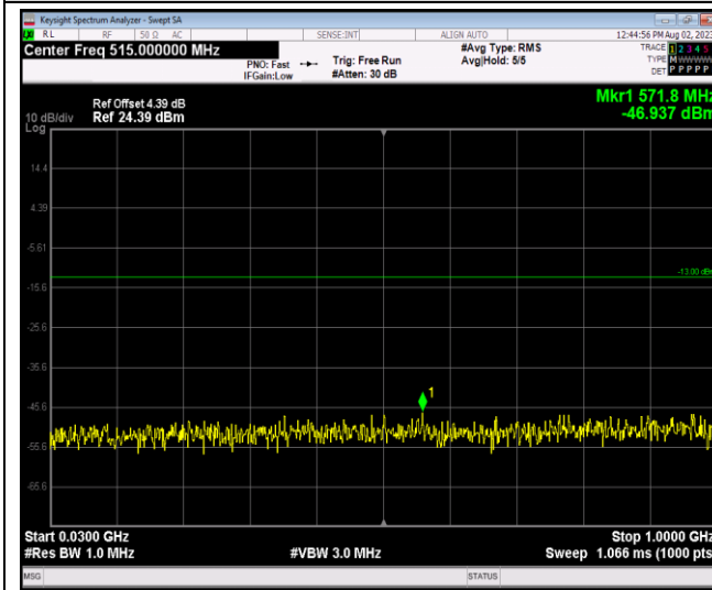
Band2-20MHz-16QAM-19100-1RB#0-Range1:30~1000MHz
