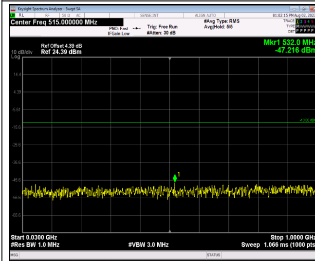
Band4-1.4MHz-64QAM-19957-1RB#0-Range1:30~1000MHz
