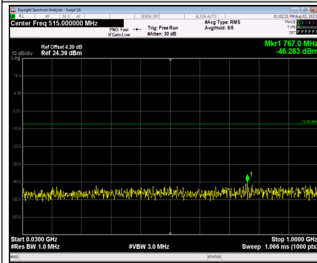
Band4-1.4MHz-QPSK-20175-1RB#0-Range1:30~1000MHz
