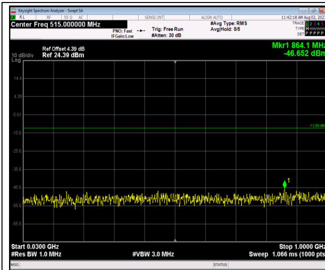
Band2-1.4MHz-64QAM-19193-1RB#0-Range1:30~1000MHz
