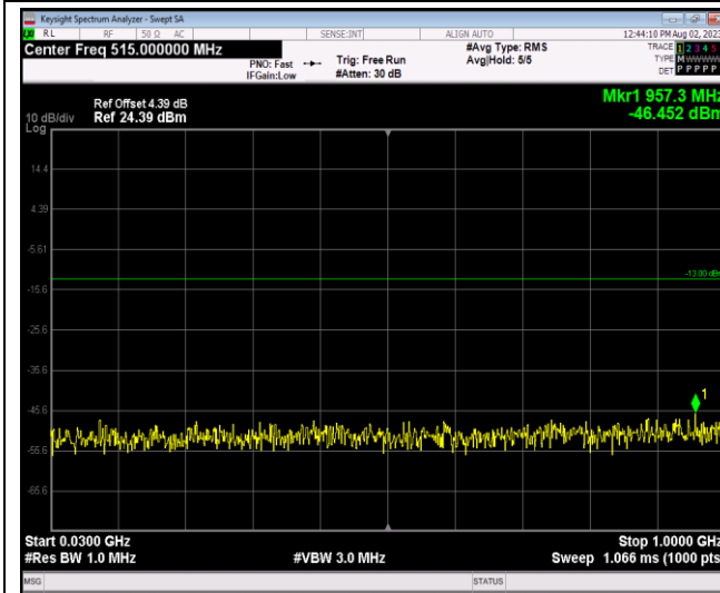
Band2-20MHz-16QAM-19100-1RB#0-Range1:30~1000MHz
