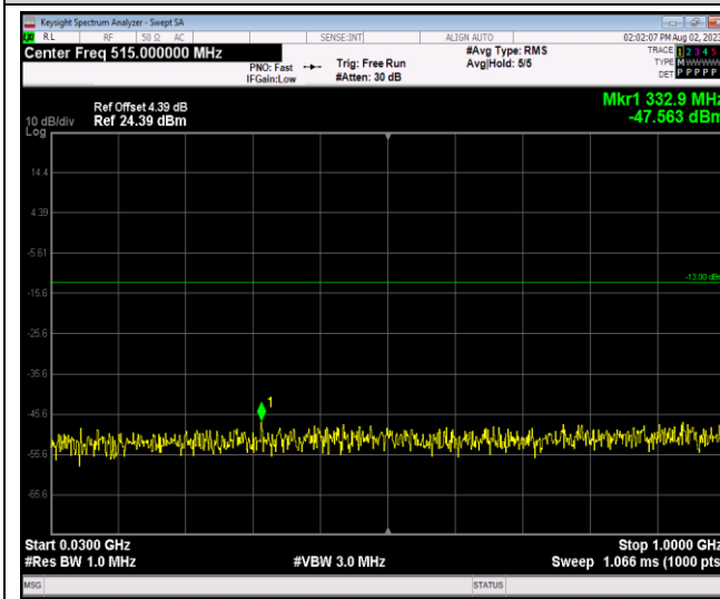
Band4-20MHz-64QAM-20175-1RB#0-Range1:30~1000MHz
