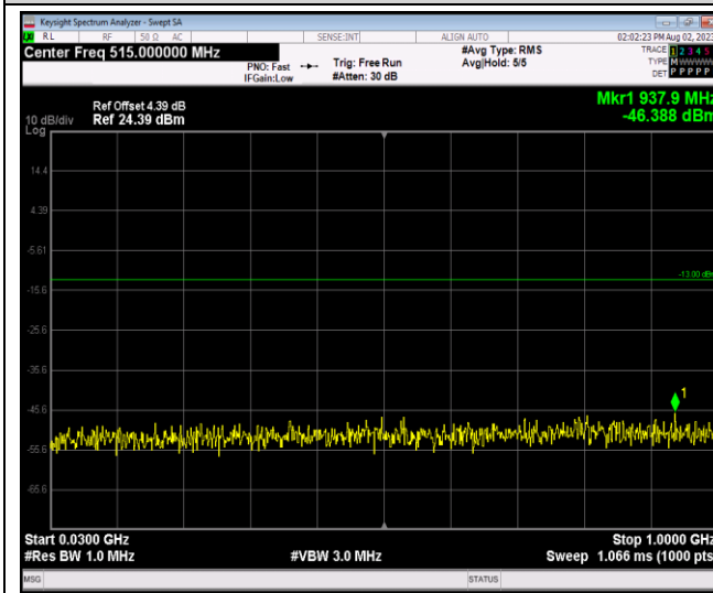
Band4-20MHz-QPSK-20300-1RB#0-Range1:30~1000MHz
