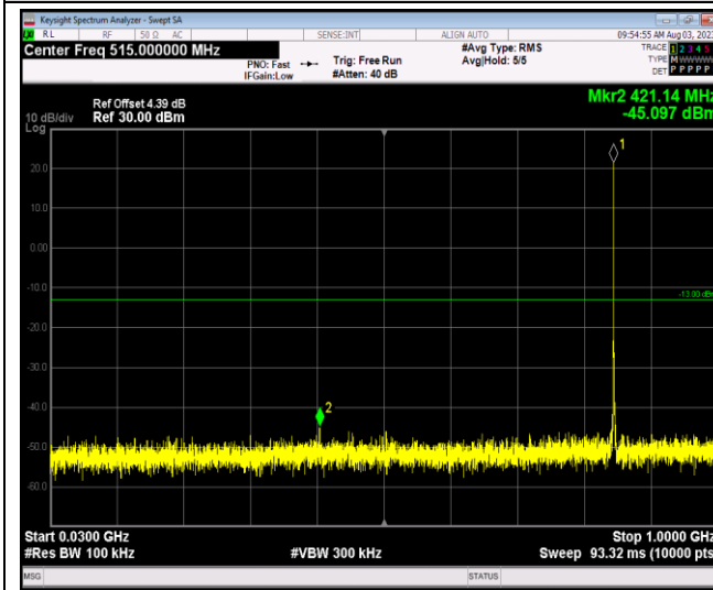
Band5-1.4MHz-64QAM-20643-1RB#0-Range1:30~1000MHz
