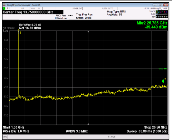
Band7-5MHz-16QAM-21100-1RB#0-Range2:1000~26500MHz
