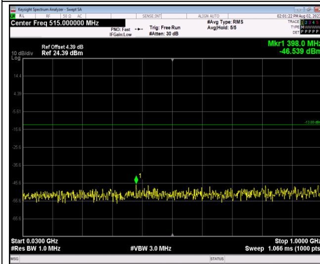
Band4-20MHz-64QAM-20175-1RB#0-Range1:30~1000MHz
