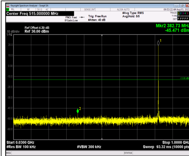
Band5-1.4MHz-64QAM-20525-1RB#0-Range1:30~1000MHz
