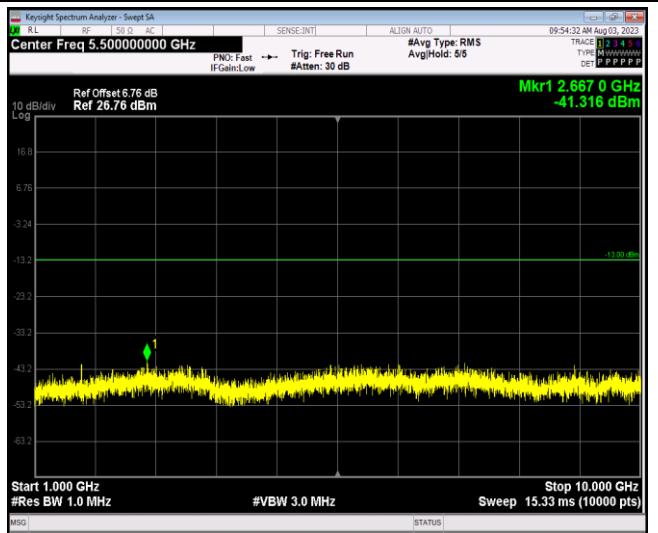
Band5-1.4MHz-16QAM-20407-1RB#0-Range2:1000~10000MHz
