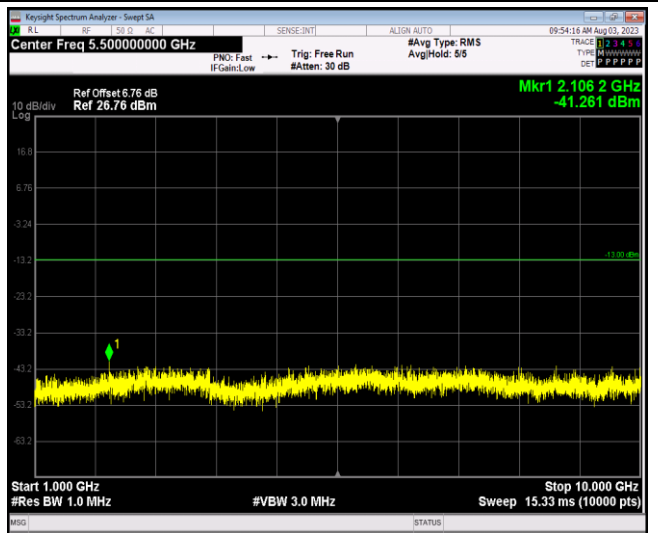
Band5-1.4MHz-64QAM-20643-1RB#0-Range2:1000~10000MHz
