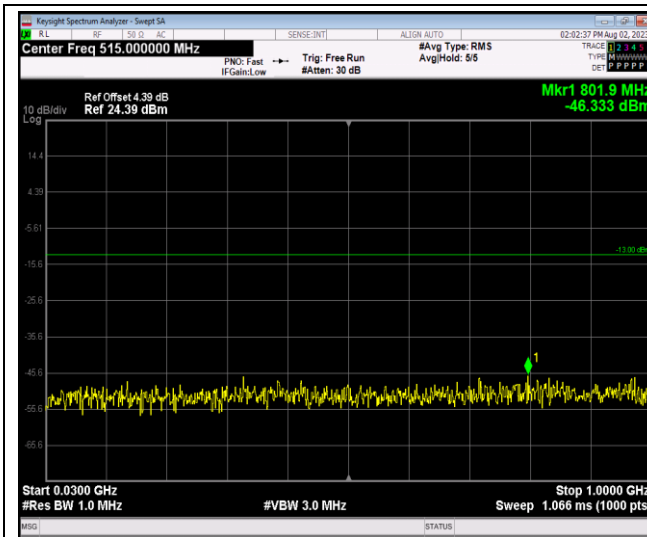
Band4-20MHz-64QAM-20050-1RB#0-Range1:30~1000MHz
