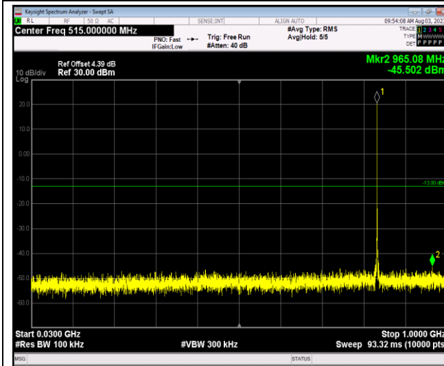
Band5-1.4MHz-64QAM-20643-1RB#0-Range1:30~1000MHz
