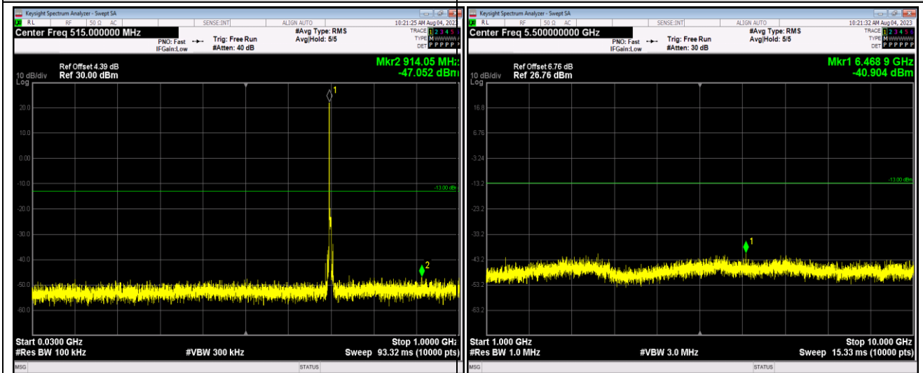
Band17-5MHz-QPSK-23790-1RB#0-Range1:30~1000MHz
