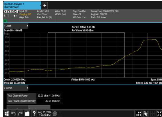
N30(5M)_DFT-s- OFDM_BPSK_Edge_1RB_Left_Low_CH_CHP_PASS
