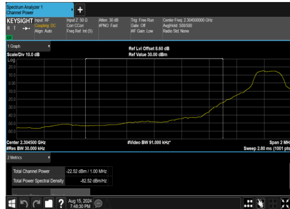
N30(5M)_DFT-s- OFDM_QPSK_Edge_1RB_Left_Low_CH_CHP_PASS
