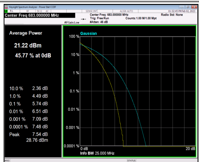
Band71-20MHz-16QAM-133322-100RB#0
