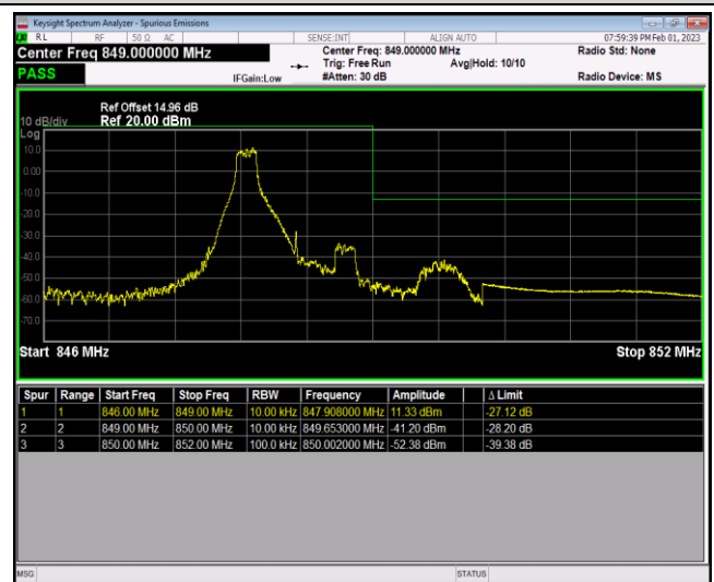
Band5-1.4MHz-16QAM-20643-6RB#0
