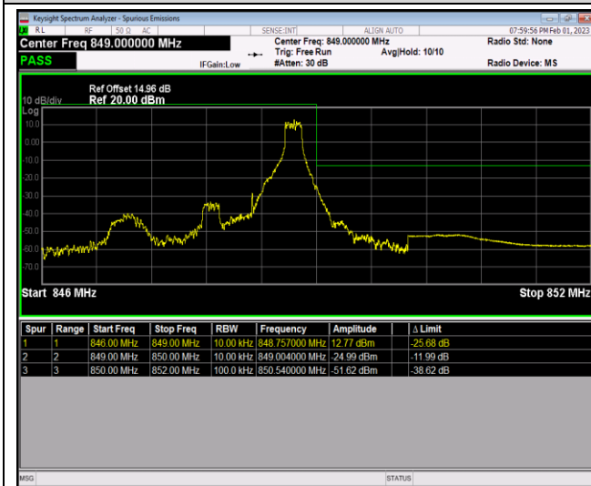
Band5-1.4MHz-16QAM-20407-1RB#0
