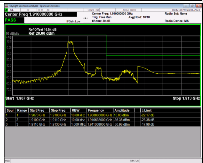
Band2-1.4MHz-16QAM-19193-6RB#0
