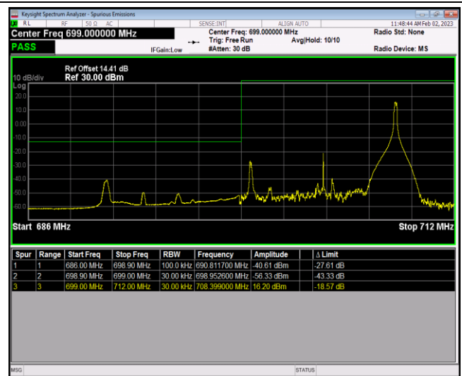
Band12-10MHz-QPSK-23130-1RB#0
