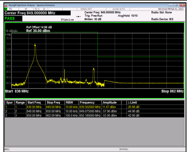
Band5-10MHz-16QAM-20600-50RB#0
