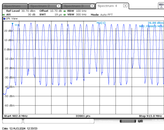
Figure 2.5.6-3: Port 1 (50 Channels)
