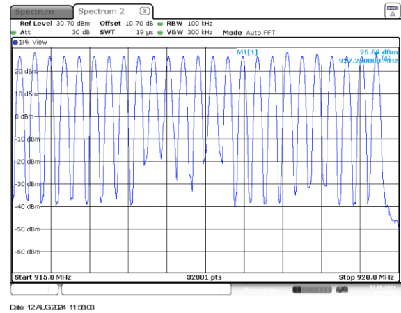
Figure 2.5.6-8: Port 3 (50 Channels)
