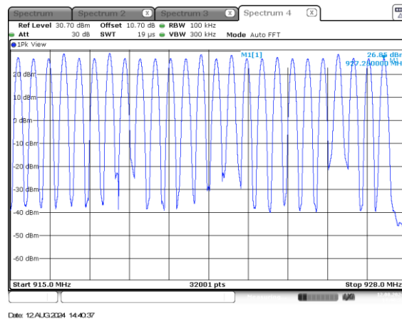
Figure 2.5.6-2: Port 0 (50 Channels)
