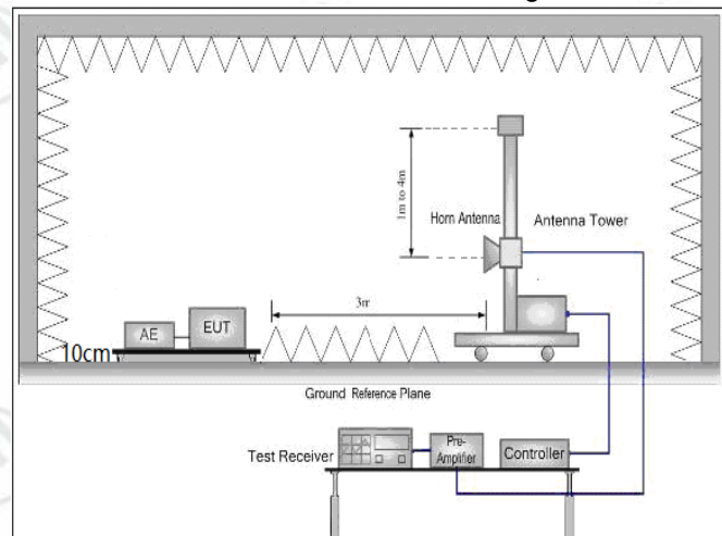
Figure 3. Above 1GHz
