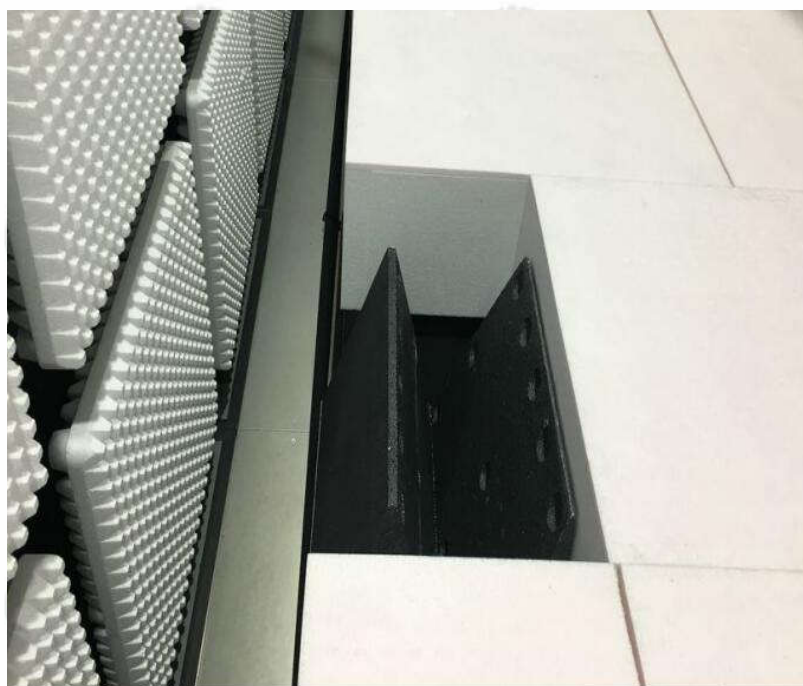
Radiated spurious emission Test Setup-4(Above 1GHz) There are absorbing materials under the ground.
