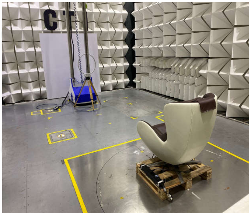
Radiated spurious emission Test Setup-1 (Below 30M)
