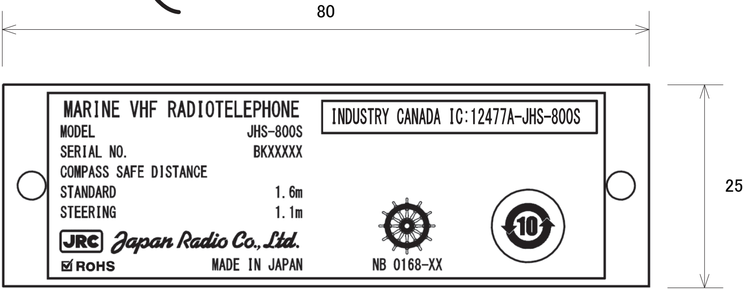
Name plate
