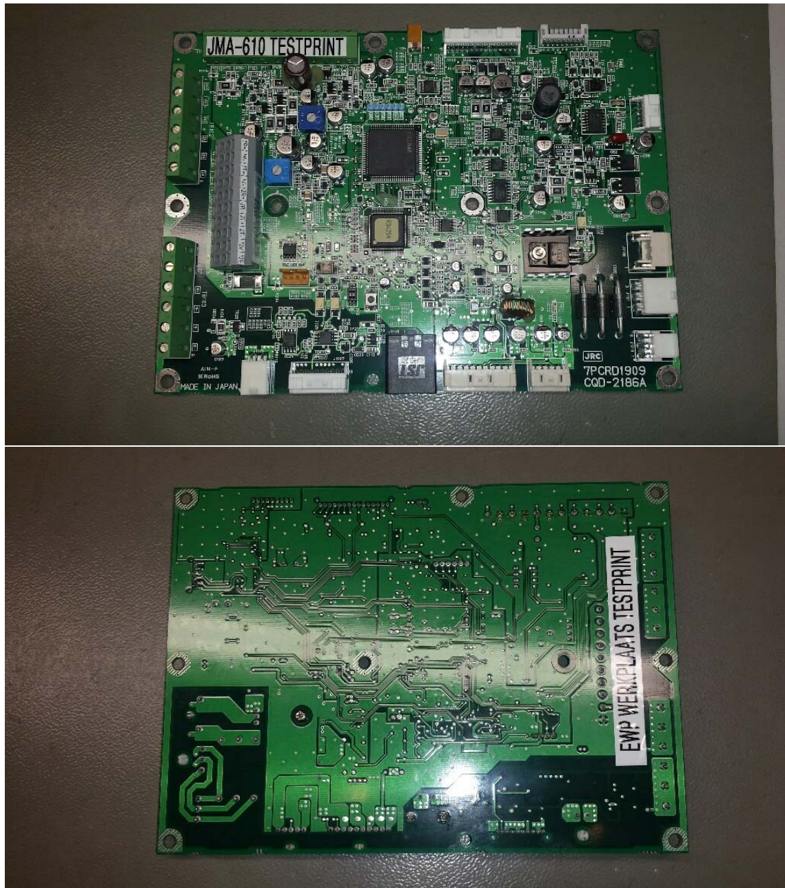
Terminal board CQD-2186
