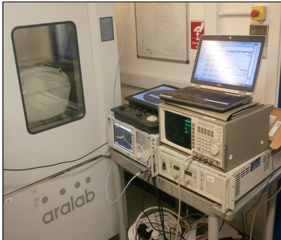
Figure 22 – Conducted Setup
