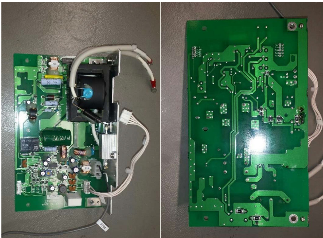
Transmitter Circuit:CPA-276
