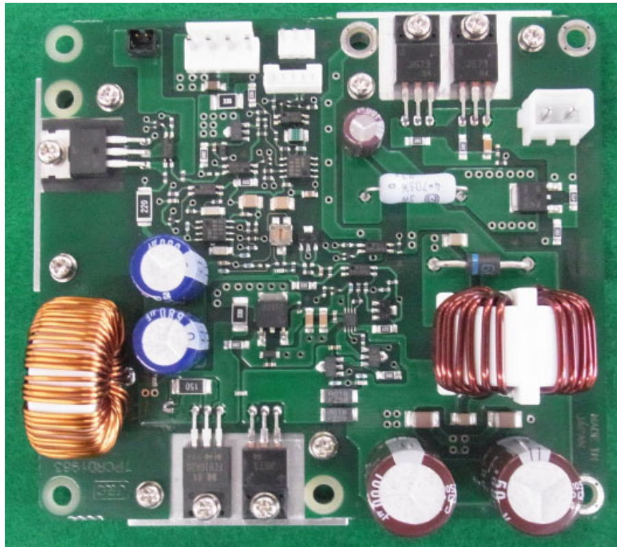
Motor Driver Circuit:CCB-705
