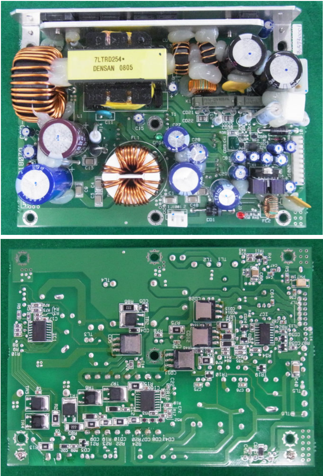
Power Supply Circuit:CBD-1783
