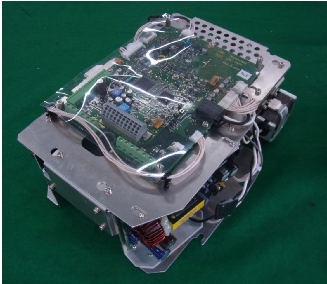
Transceiver Unit:NZT-18
