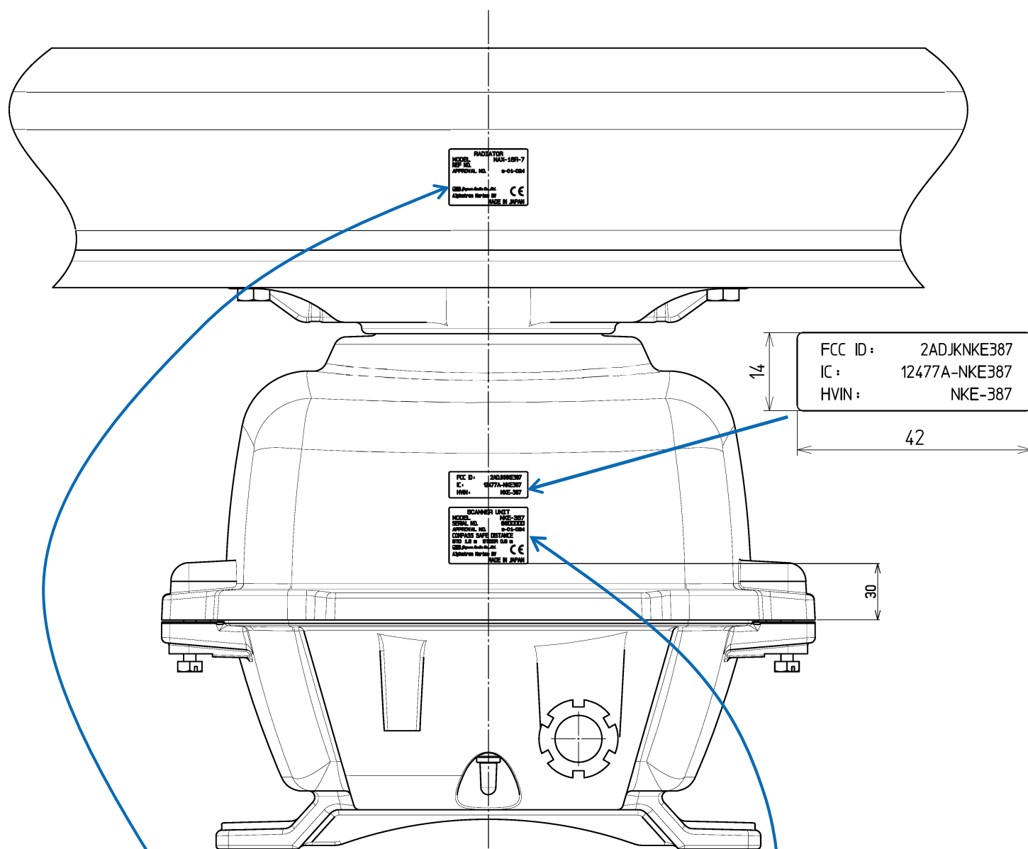
BACK VIEW
