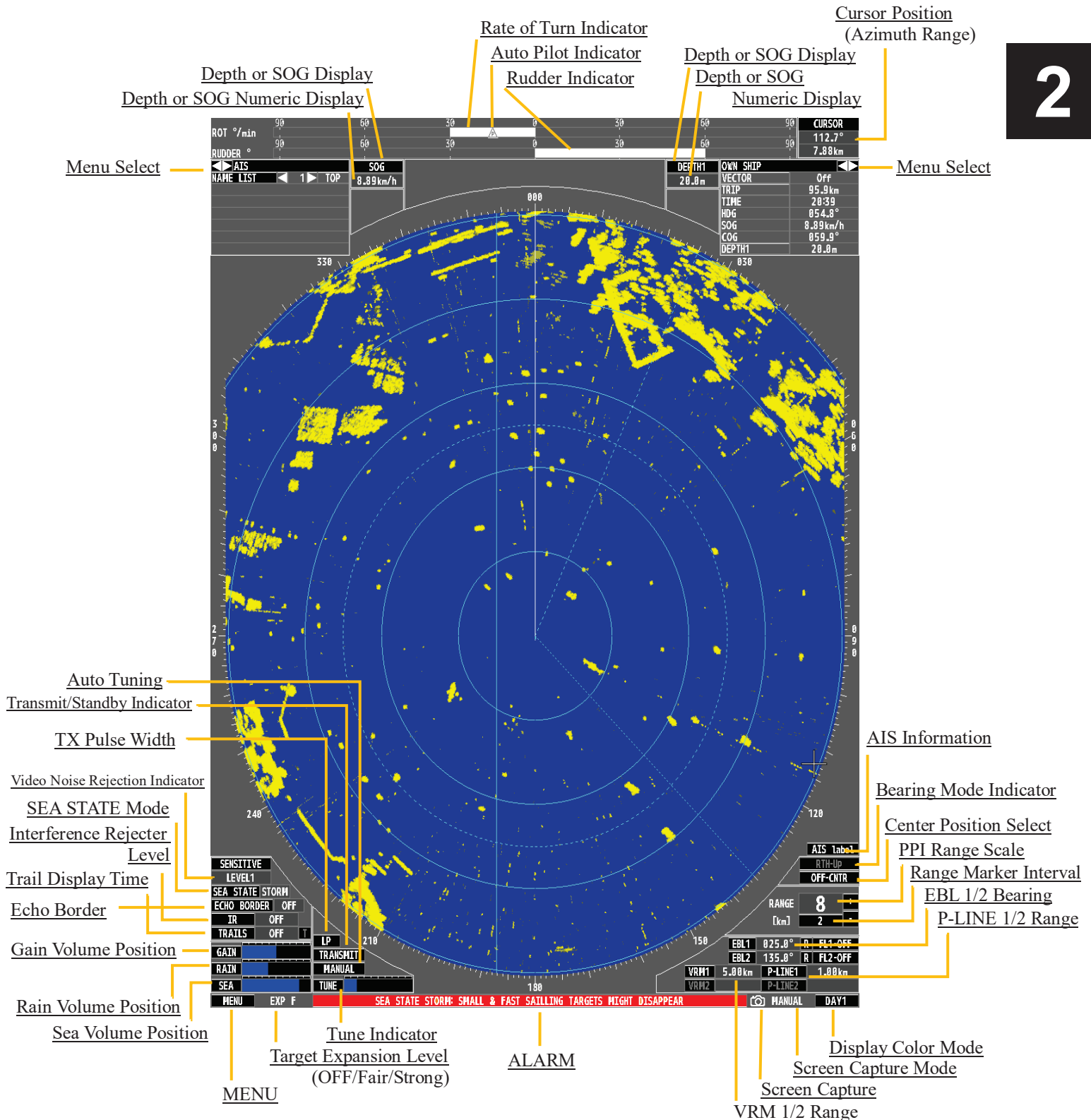
FIG 2.1 DISPLAY &amp; READOUTS
