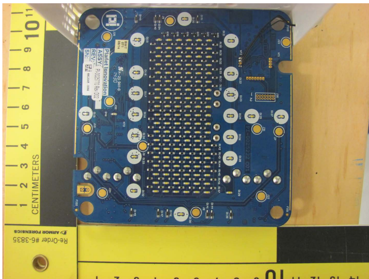
Figure 3: EUT internal photo – rear view
