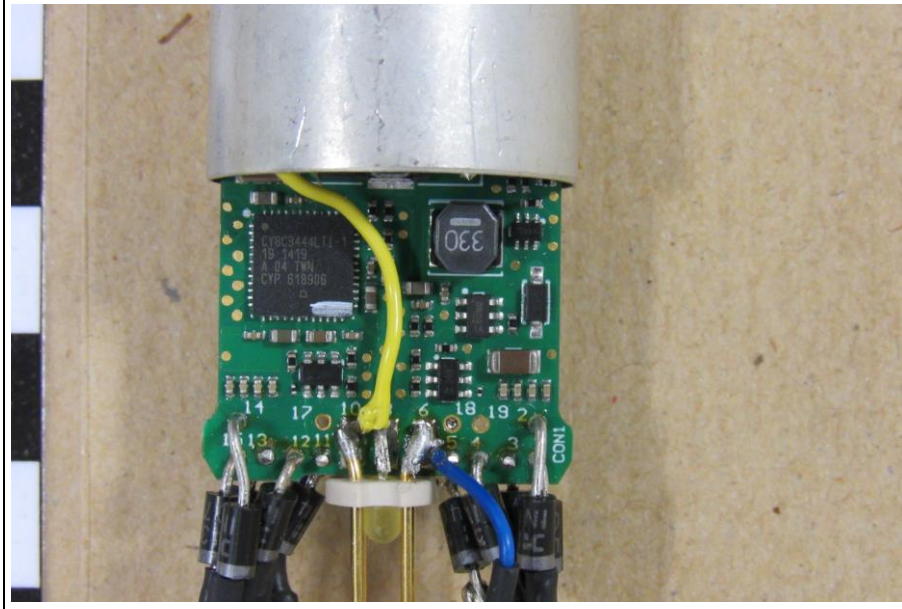
PCB Detail
