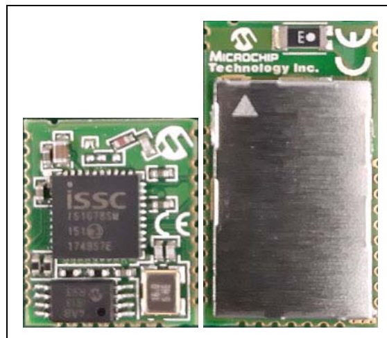
FIGURE 1: BM78 MODULE
