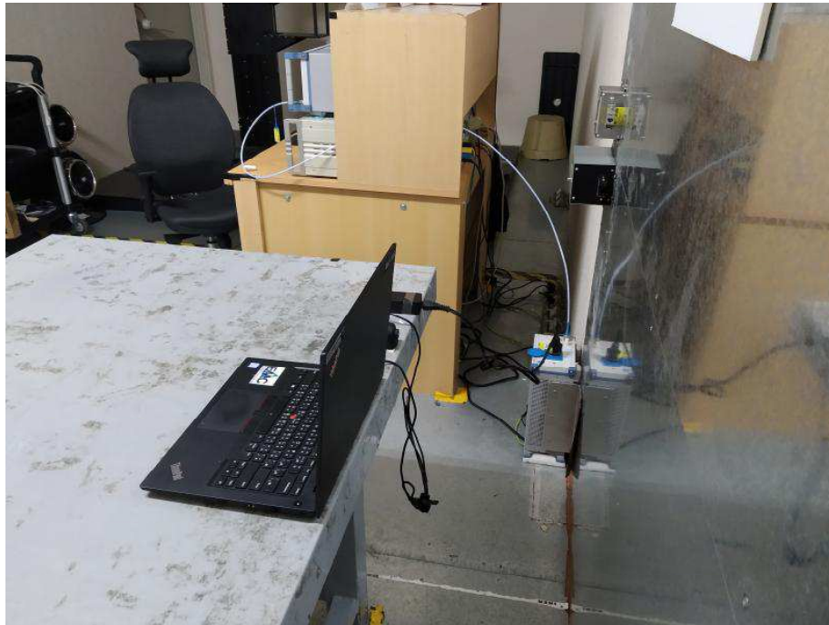
Photograph 10: Set-up for Mains Conducted testing (Front View)
