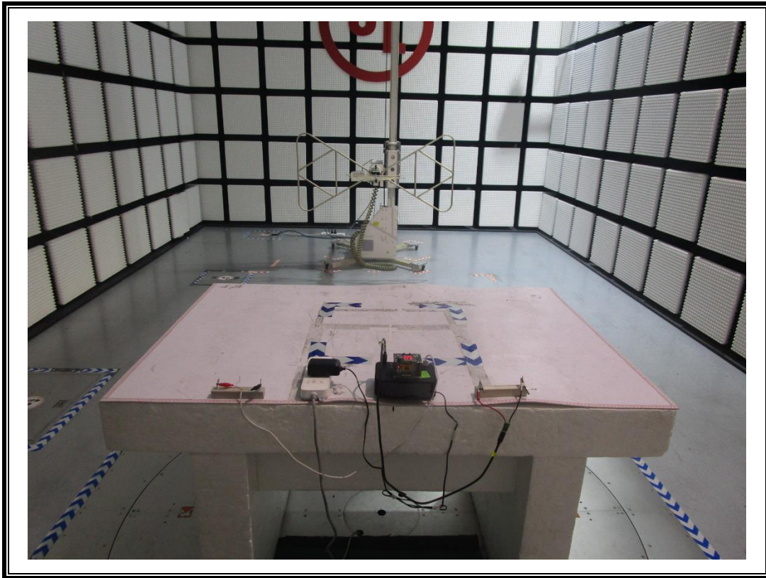
RADIATED EMISSIONS MEASUREMENT SETUP (30MHz ~ 1 GHz)
