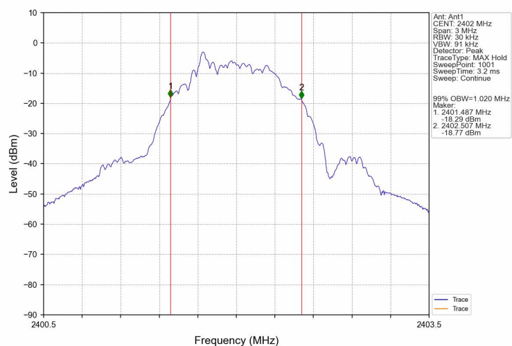
99%_Occupied_Bandwidth_NVNT_ANT1_1Mbps_2402
