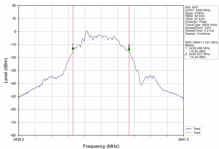
99%_Occupied_Bandwidth_NVNT_ANT1_1Mbps_2440
