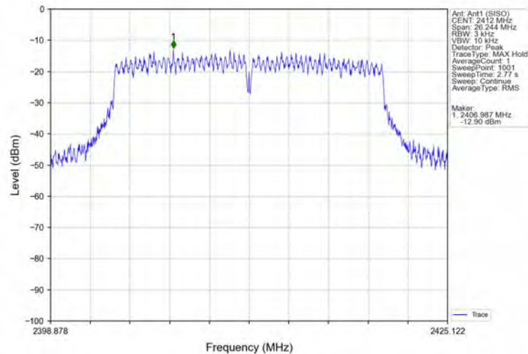
Power_Spectral_Density_NVNT_ANT1_802_11n(HT20)_2412
