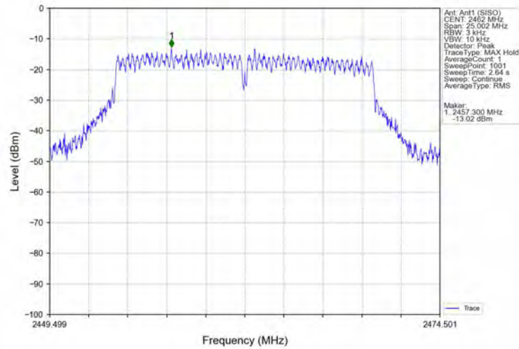
Power_Spectral_Density_NVNT_ANT1_802_11g_2462
