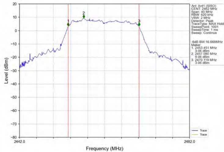
-6dB_Bandwidth_NVNT_ANT1_802_11g_2462
