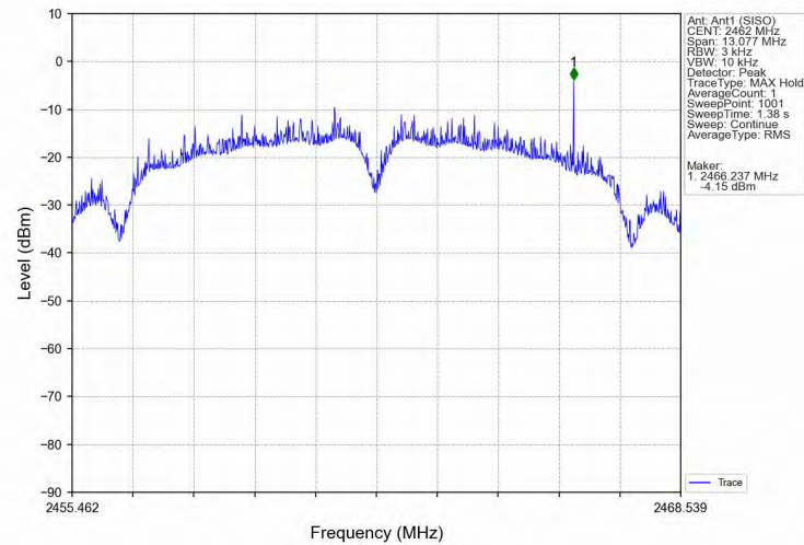
Power_Spectral_Density_NVNT_ANT1_802_11b_2462
