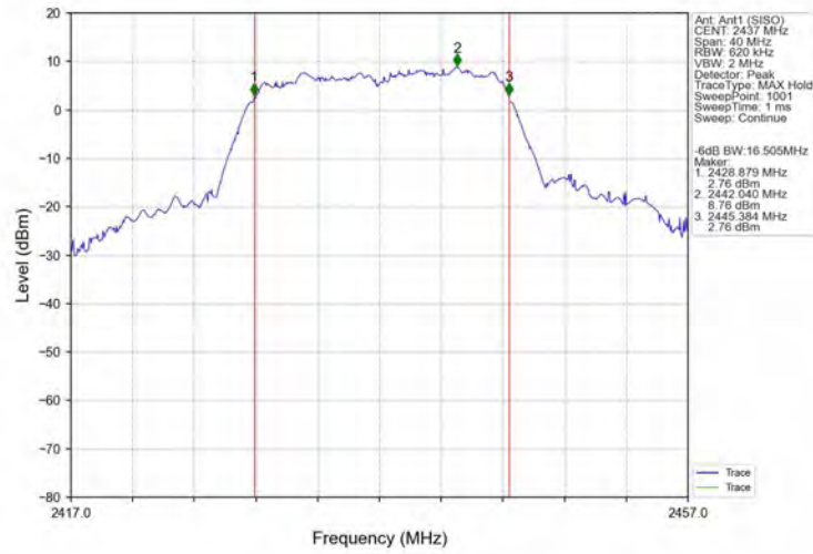
-6dB_Bandwidth_NVNT_ANT1_802_11g_2437
