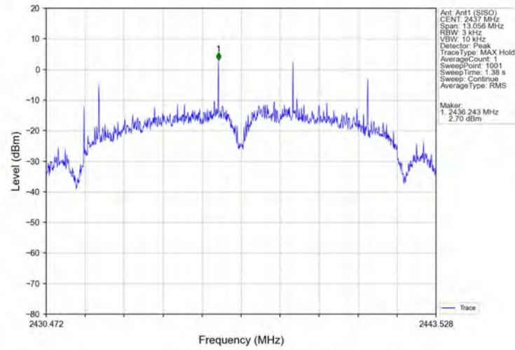
Power_Spectral_Density_NVNT_ANT1_802_11b_2437
