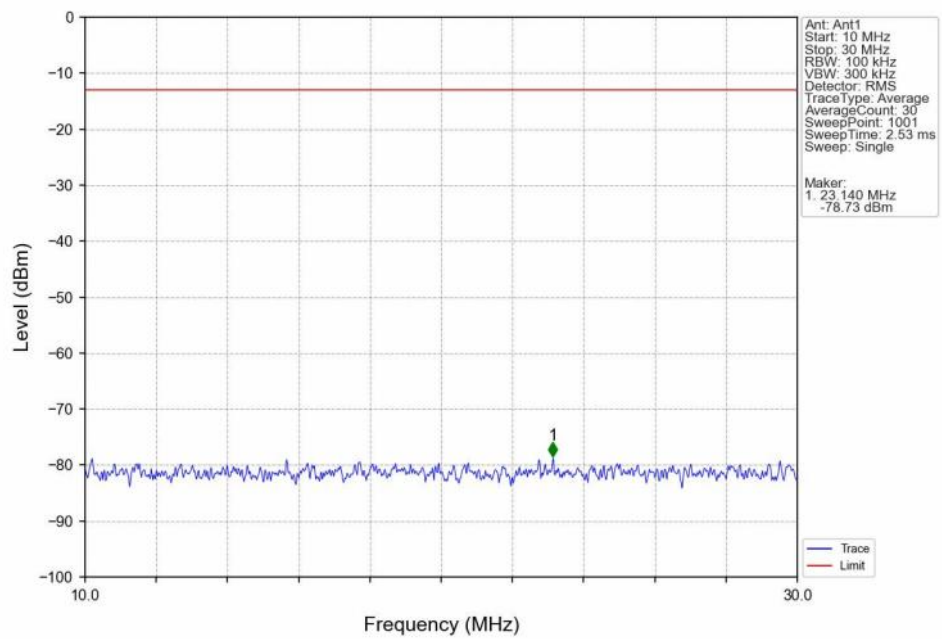
Band17_10MHz_16QAM_LCH_709MHz_RB_1_0_NTNV
