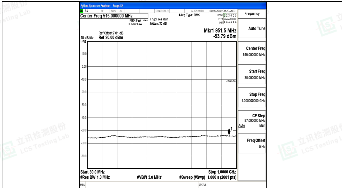
Band25_15MHz_16QAM_26365_1RB#0_30~1000_30~1000
