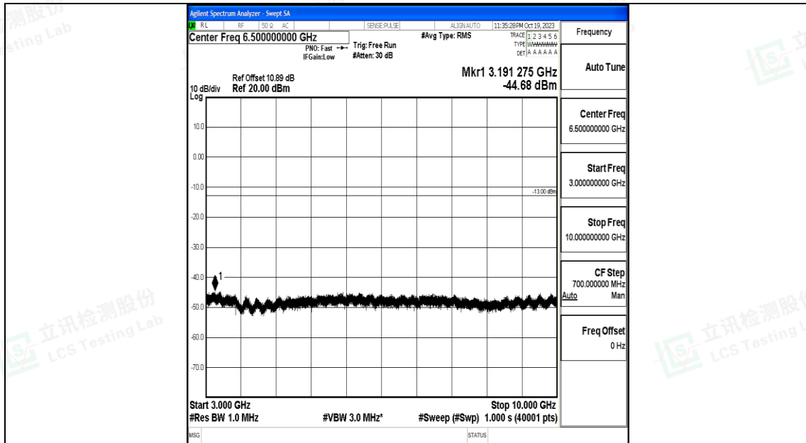
Band26_15MHz_QPSK_26965_1RB#0_3000~10000_3000~10000
