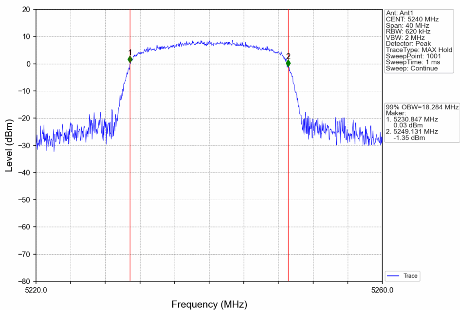
802.11ac(VHT20)_HCH_5240MHz_Ant1_NTNV
