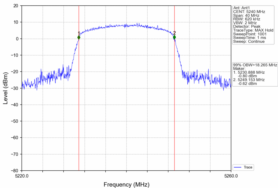
802.11a_HCH_5240MHz_Ant1_NTNV
