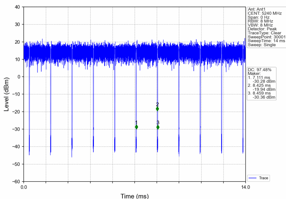
802.11ac(VHT20)_HCH_5240MHz_Ant1_NTNV
