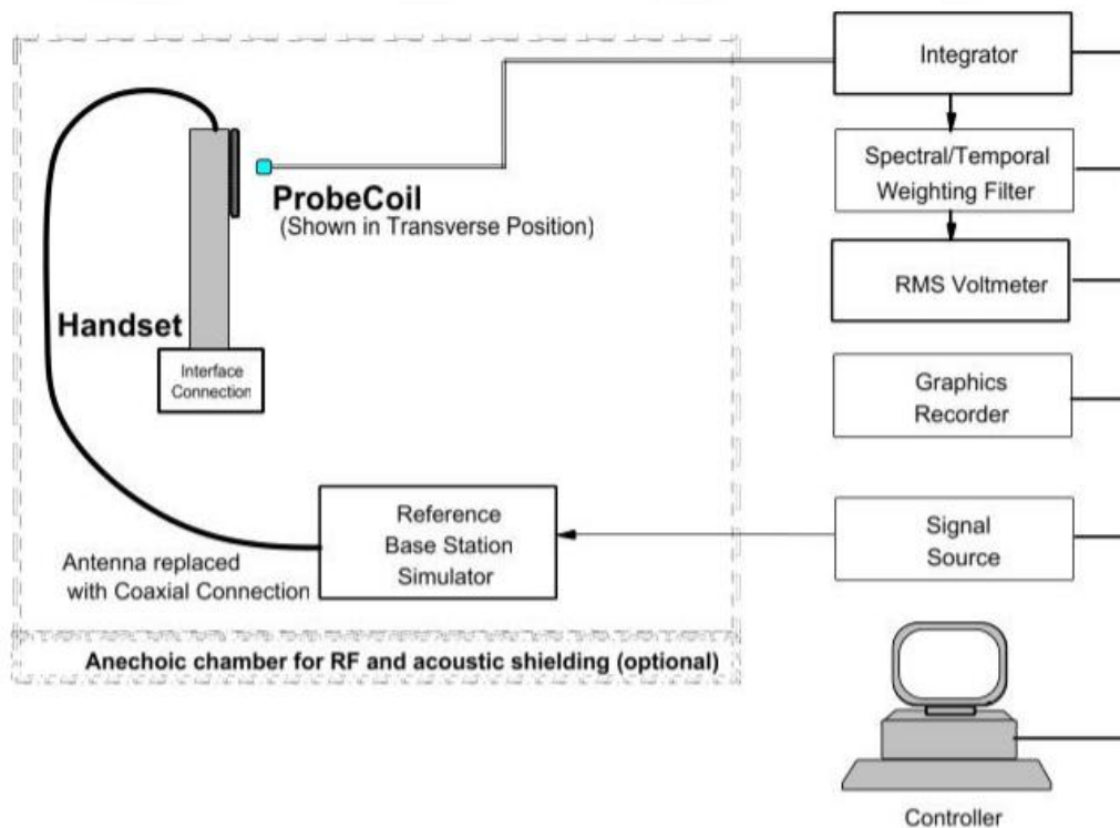
Fig. 3. T-coil measurement test setup
