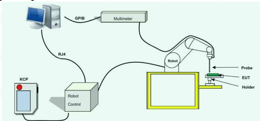
MVG HAC System Diagram
