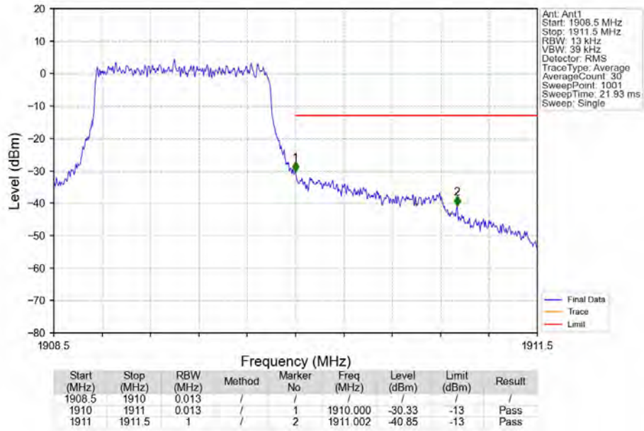
Band2_1.4MHz_QPSK_HCH_1909.3MHz_RB_6_0_NTNV
