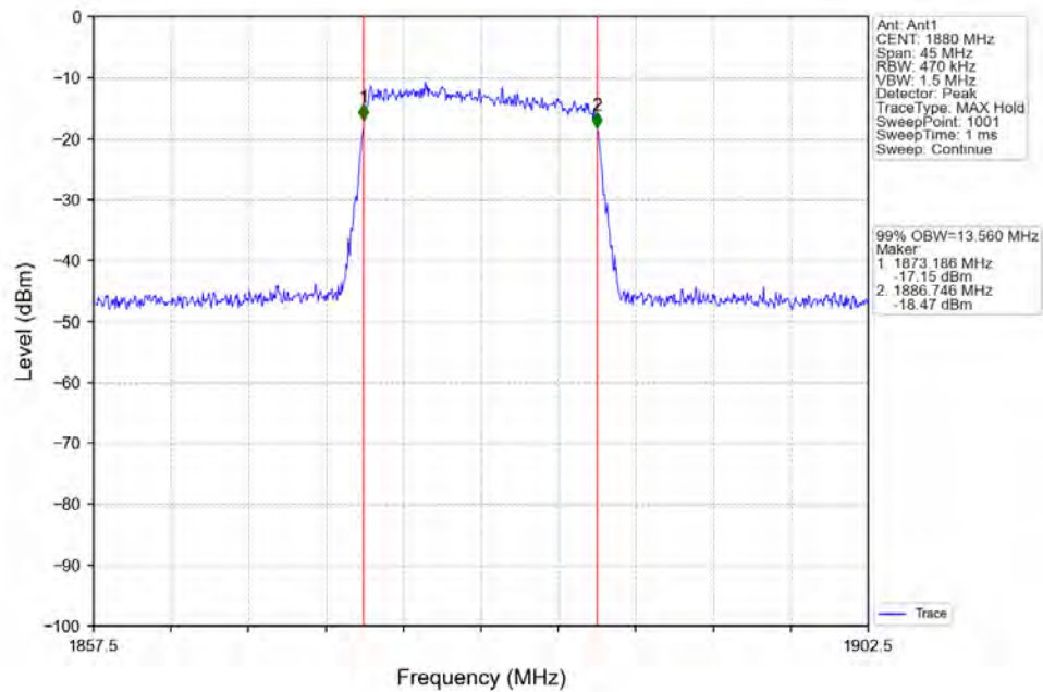
Band2_15MHz_QPSK_MCH_1880MHz_RB_75_0_NTNV
