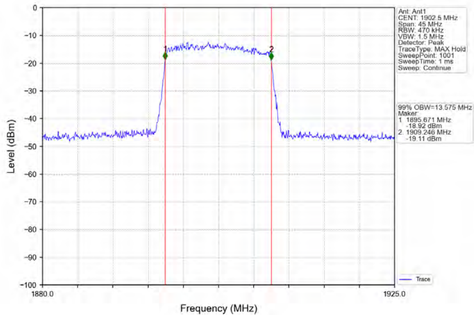
Band2_15MHz_16QAM_HCH_1902.5MHz_RB_75_0_NTNV
