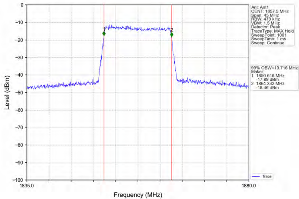
Band2_15MHz_16QAM_LCH_1857.5MHz_RB_75_0_NTNV
