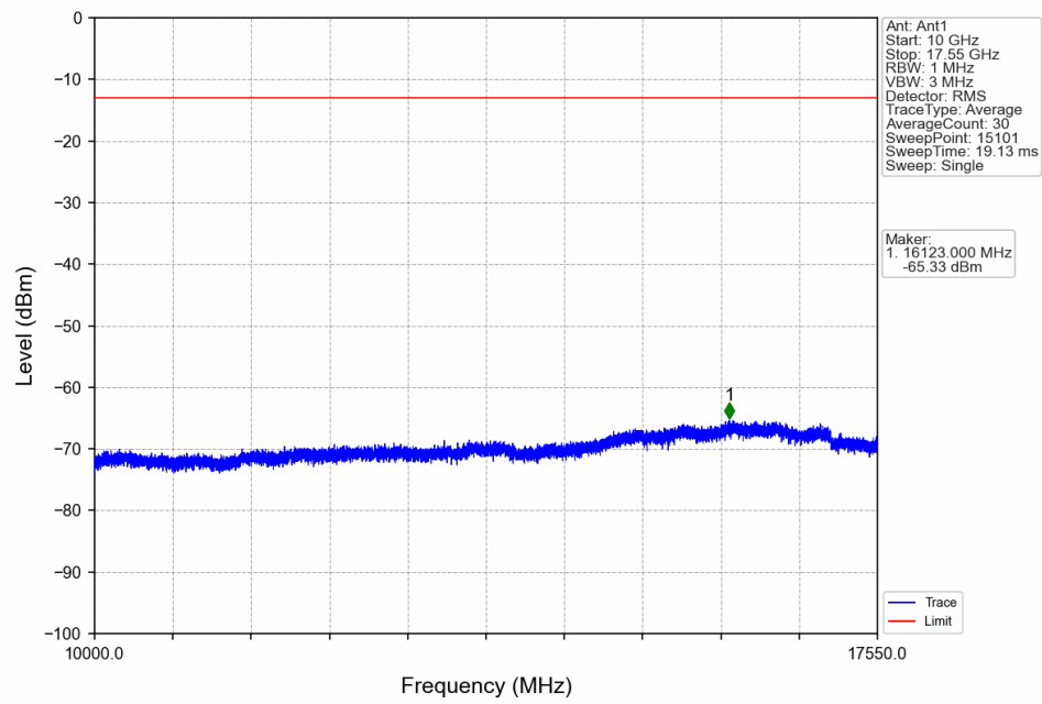
Band4_HSUPA_HCH_1752.6MHz_Subtest 1_NTNV
