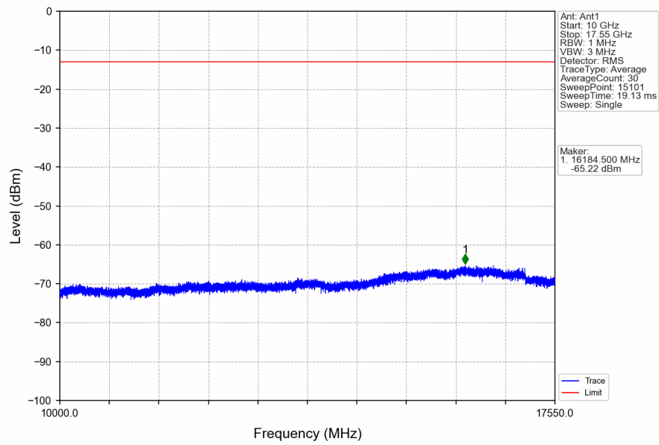
Band4_HSDPA_HCH_1752.6MHz_Subtest 1_NTNV
