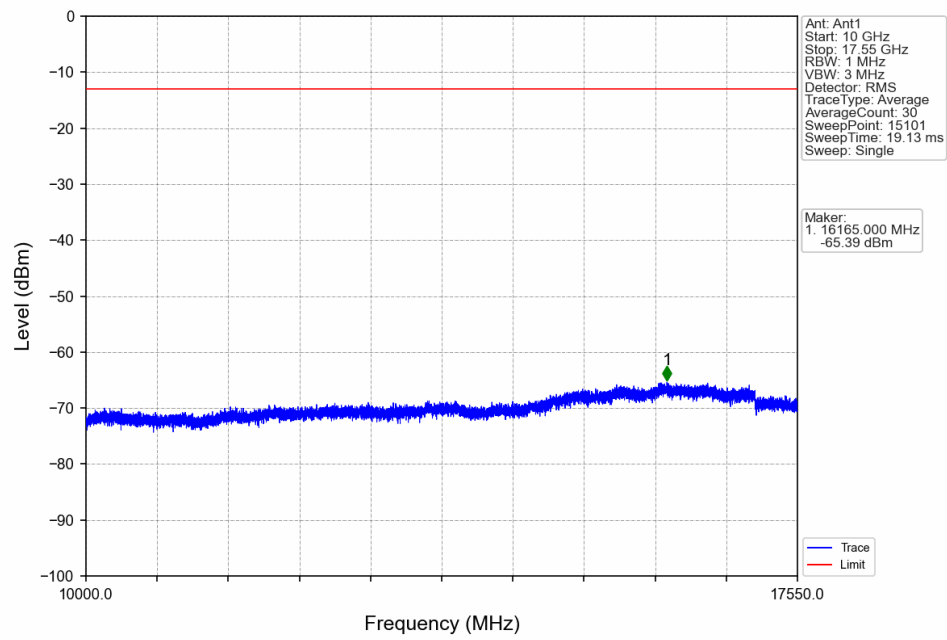
Band4_HSDPA_MCH_1732.6MHz_Subtest 1_NTNV
