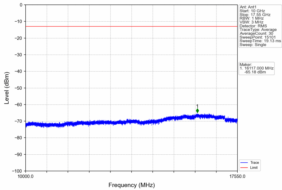
Band4_HSUPA_MCH_1732.6MHz_Subtest 1_NTNV
