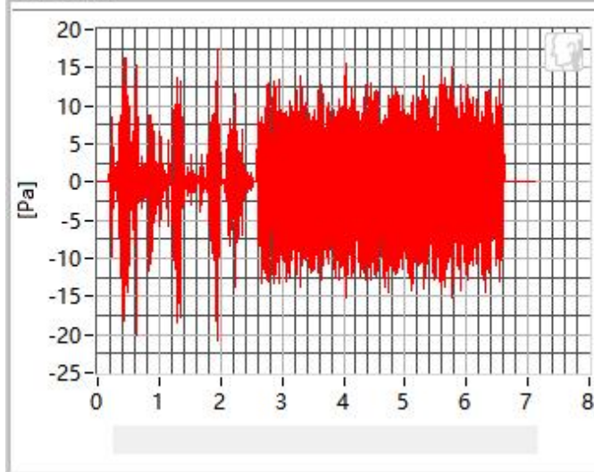
2500 Hz NB
