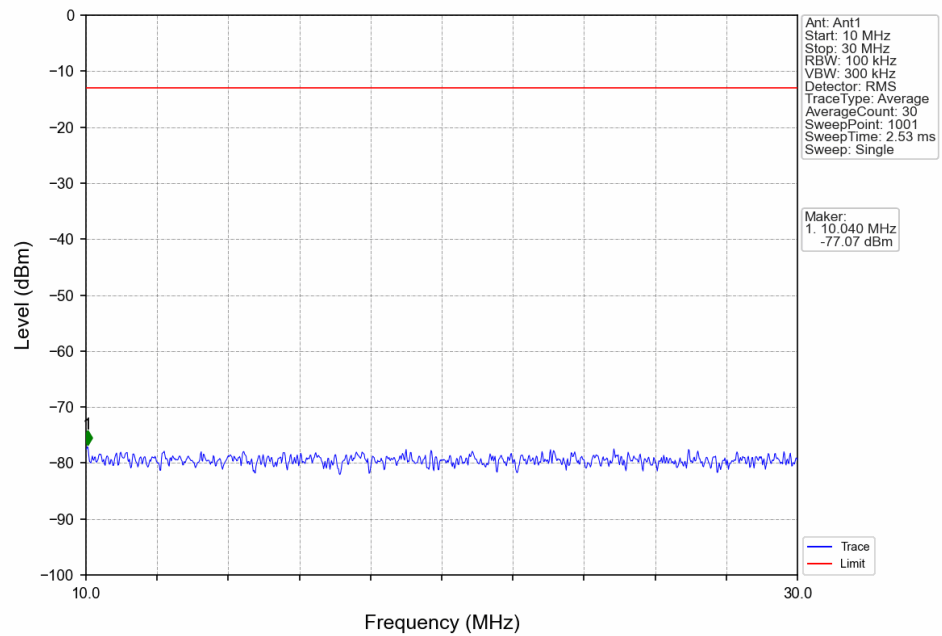
Band5_5MHz_QPSK_LCH_826.5MHz_RB_1_0_NTNV
