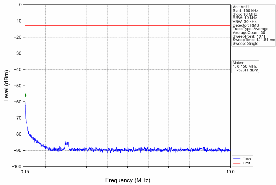
Band5_5MHz_QPSK_LCH_826.5MHz_RB_1_0_NTNV
