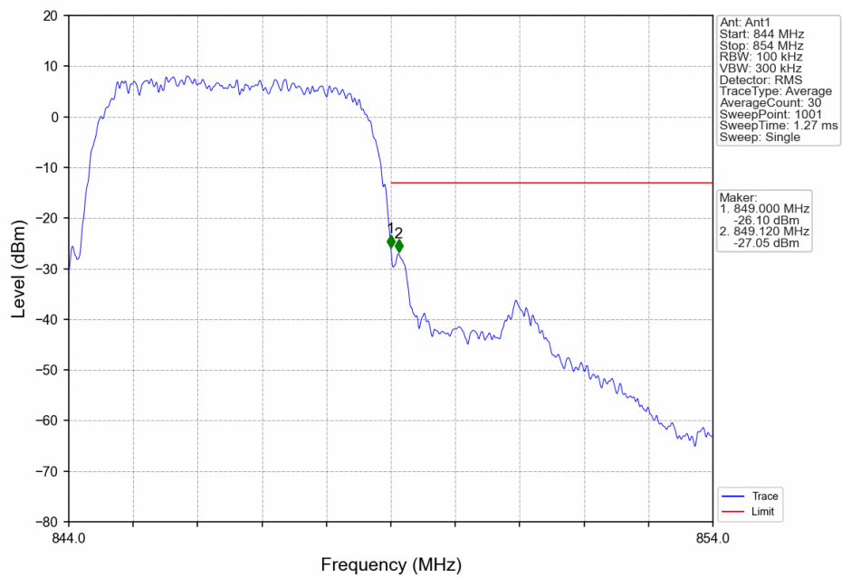
Band5_RMC_HCH_846.6MHz_12.2kbps RMC_NTNV
