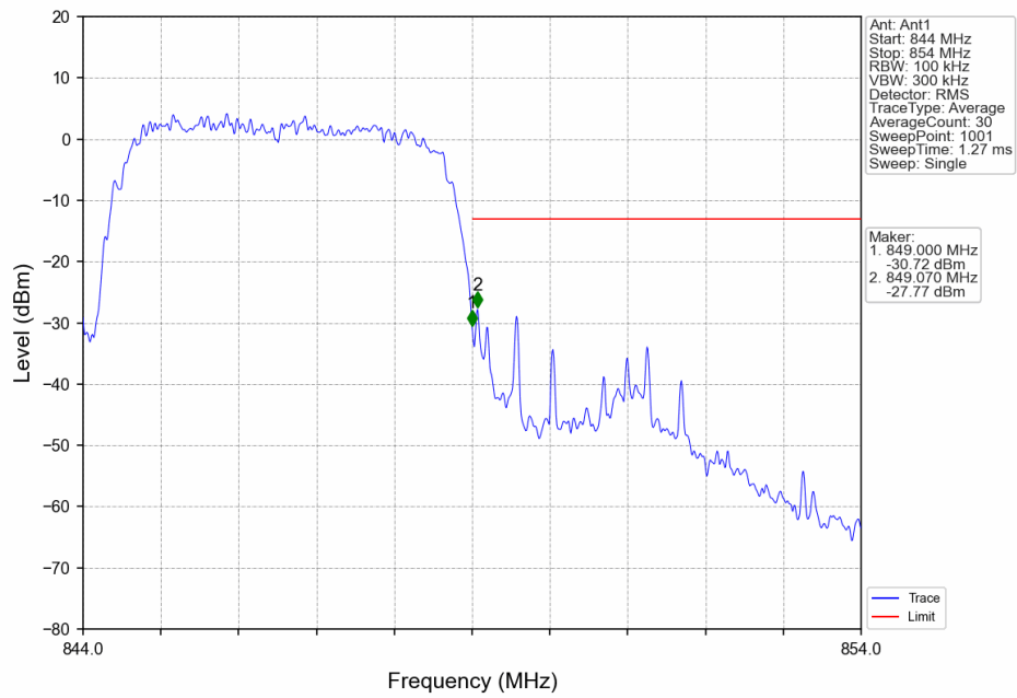
Band5_HSUPA_HCH_846.6MHz_Subtest 1_NTNV
