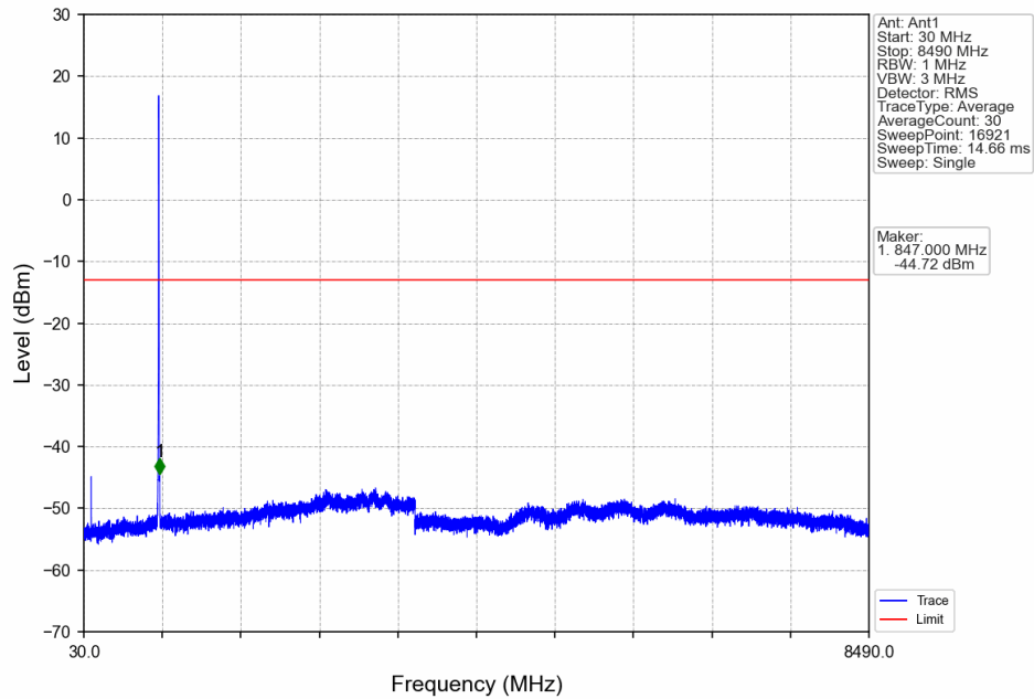
Band5_RMC_HCH_846.6MHz_12.2kbps RMC_NTNV
