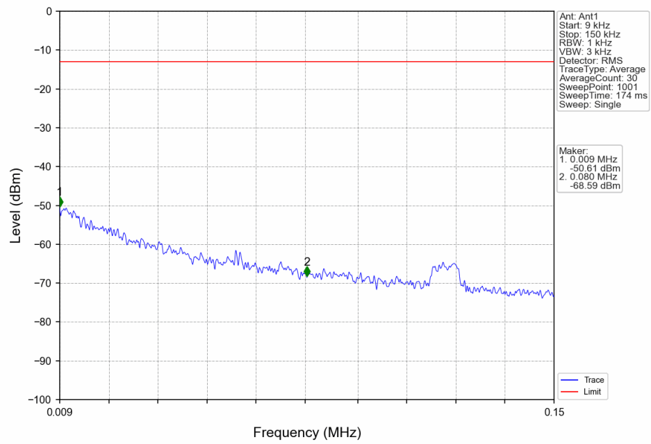
Band12_3MHz_16QAM_MCH_707.5MHz_RB_1_0_NTNV
