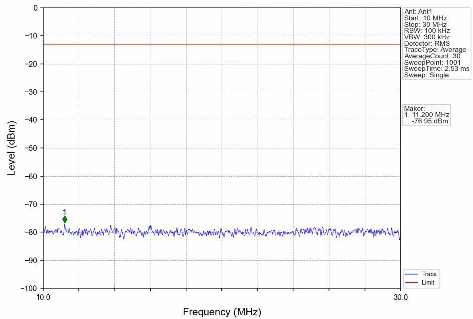
Band12_1.4MHz_16QAM_LCH_699.7MHz_RB_1_0_NTNV
