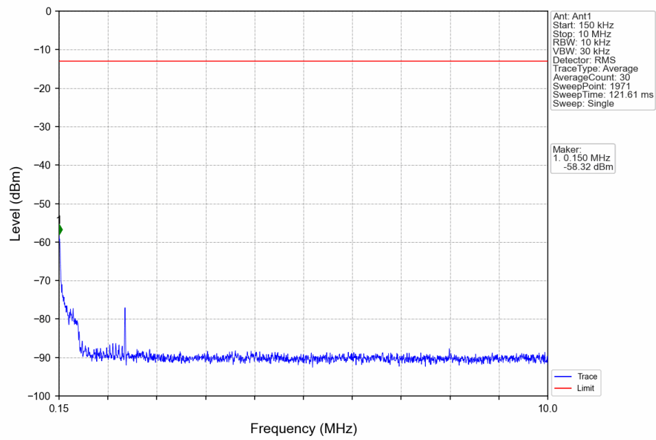
Band12_1.4MHz_16QAM_LCH_699.7MHz_RB_1_0_NTNV
