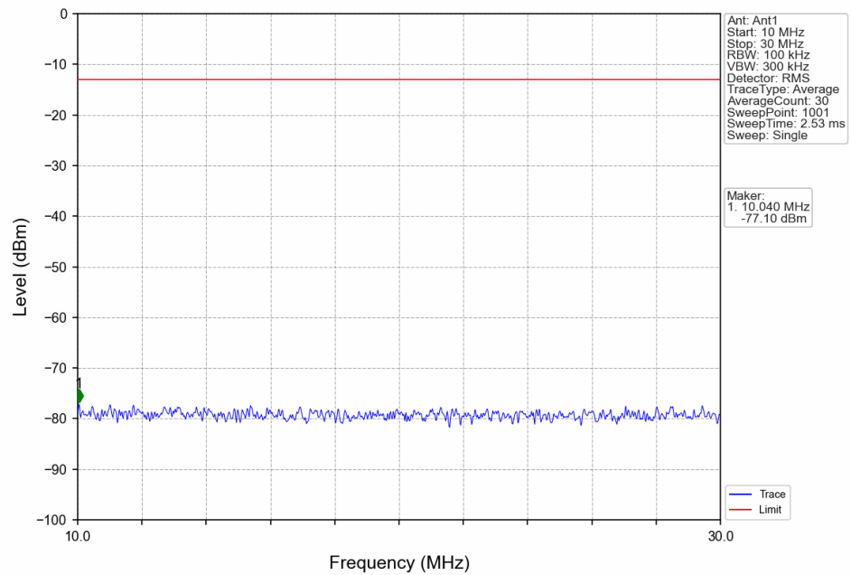
Band26a_3MHz_QPSK_LCH_815.5MHz_RB_1_0_NTNV
