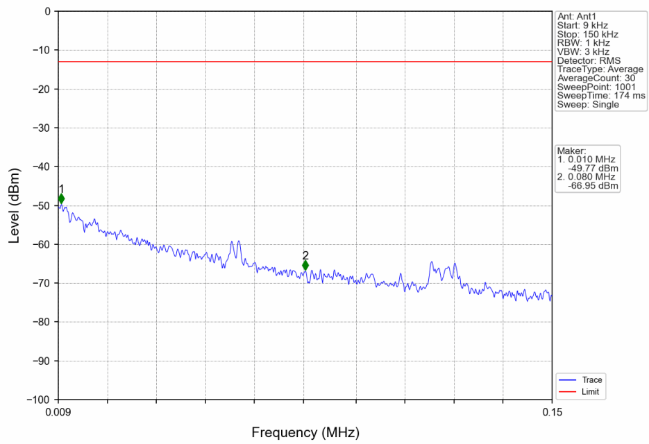
Band26c_15MHz_16QAM_MCH_831.5MHz_RB_1_0_NTNV
