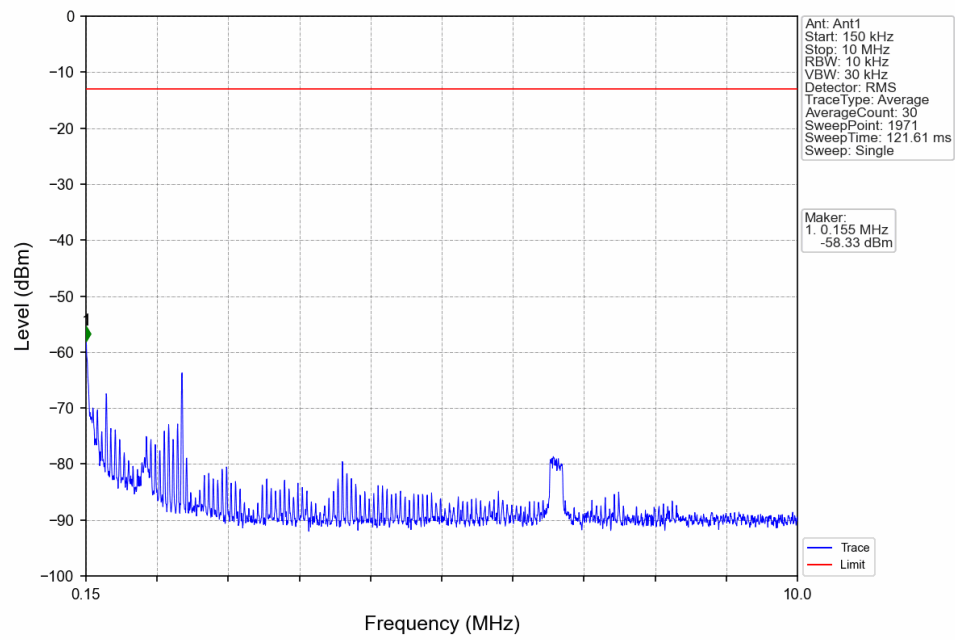
Band26c_15MHz_16QAM_LCH_821.5MHz_RB_1_0_NTNV
