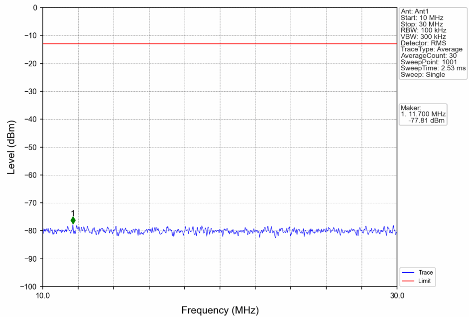
Band26c_15MHz_16QAM_LCH_821.5MHz_RB_1_0_NTNV
