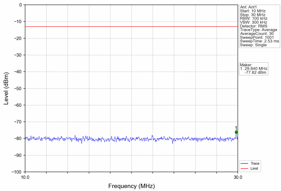
Band26c_15MHz_16QAM_MCH_831.5MHz_RB_1_0_NTNV
