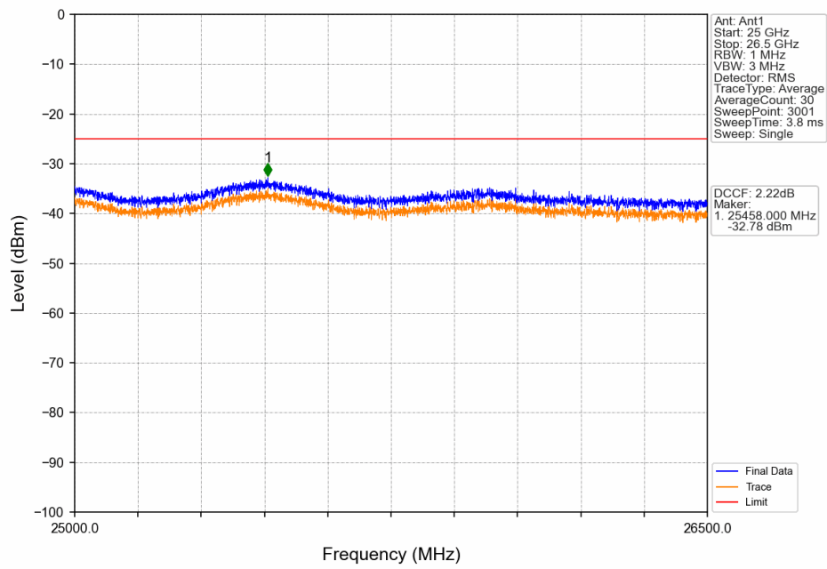
Band41_15MHz_16QAM_LCH_2503.5MHz_RB_75_0_NTNV
