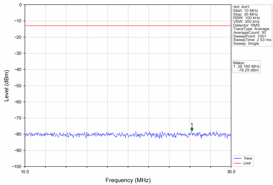
Band66_1.4MHz_16QAM_LCH_1710.7MHz_RB_1_0_NTNV
