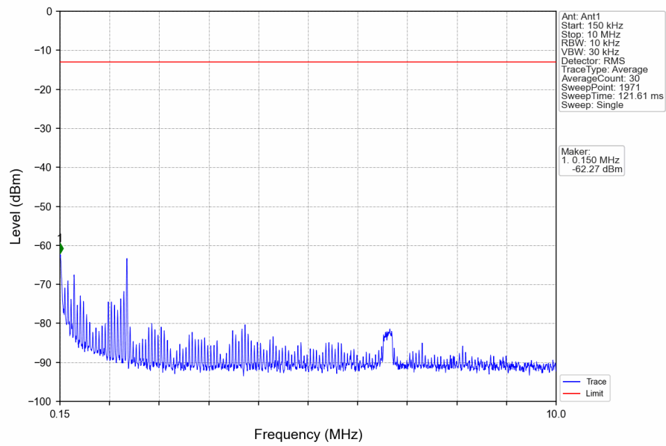
Band66_15MHz_16QAM_HCH_1772.5MHz_RB_1_0_NTNV
