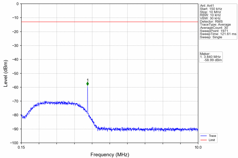
Band4_RMC_HCH_1752.6MHz_12.2kbps RMC_NTNV
