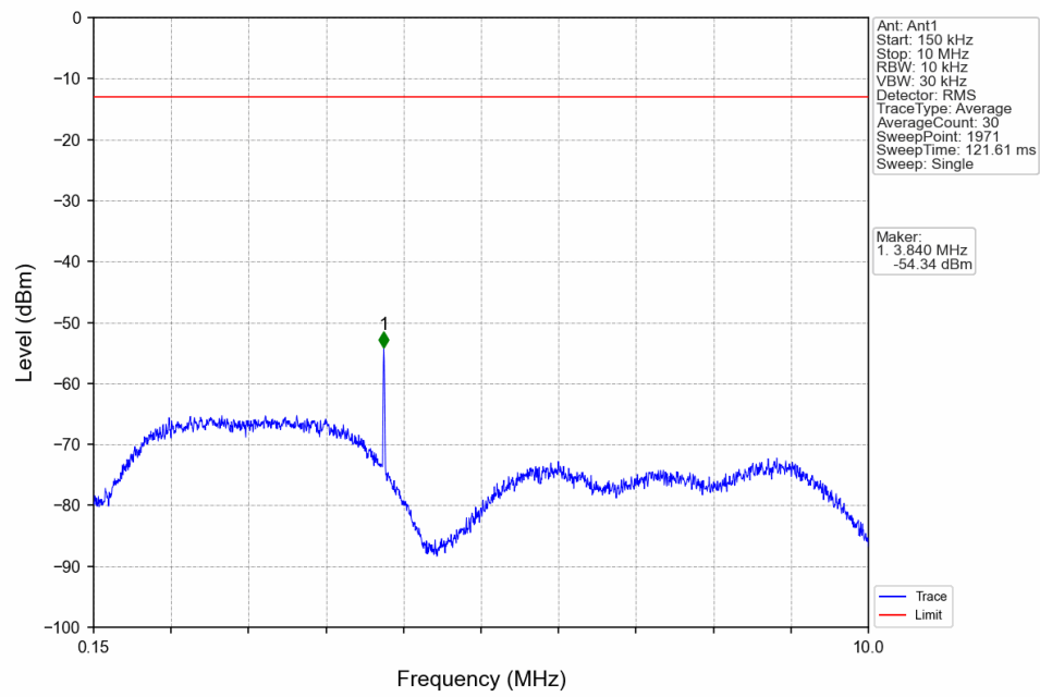
Band4_RMC_LCH_1712.4MHz_12.2kbps RMC_NTNV
