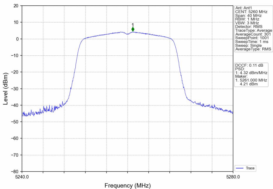
802.11ac(VHT20)_LCH_5260MHz_Ant1_NTNV
