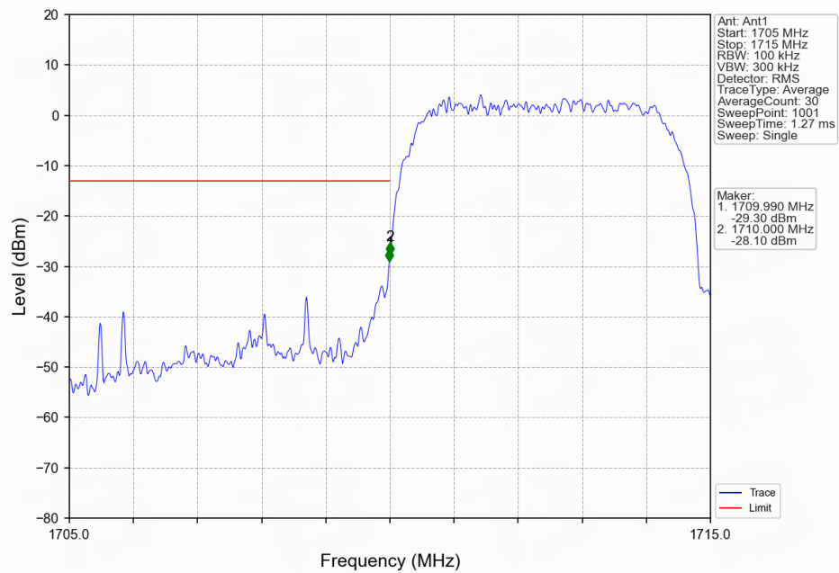
Band4 HSUPA LCH 1712.4MHz Subtest 1_NTNV
