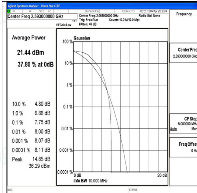
Band41-10MHz-QPSK-40620-1RB#0-PASS
