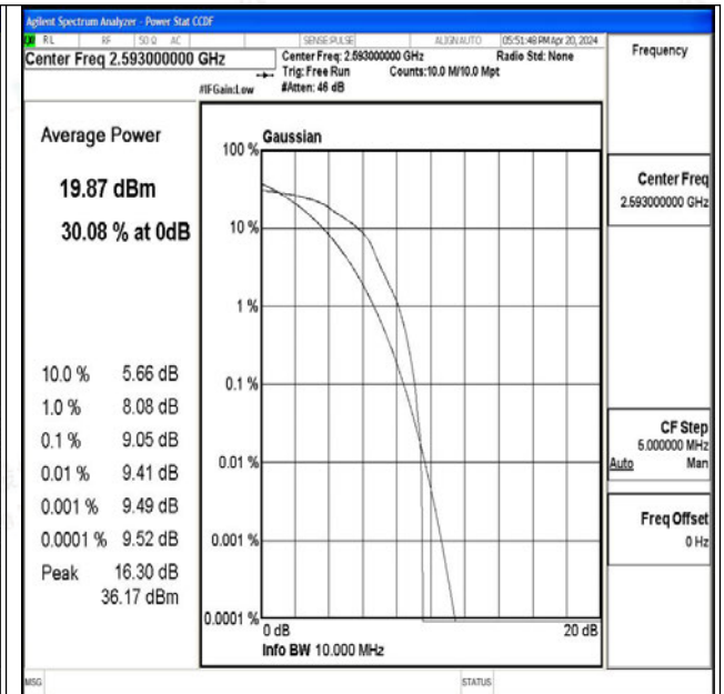
Band41-10MHz-16QAM-40620-1RB#0-PASS
