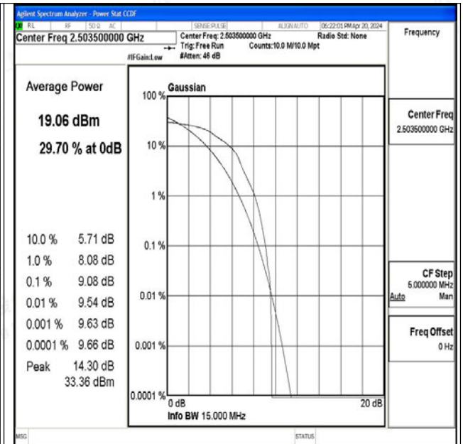
Band41-15MHz-16QAM-39725-1RB#0-PASS
