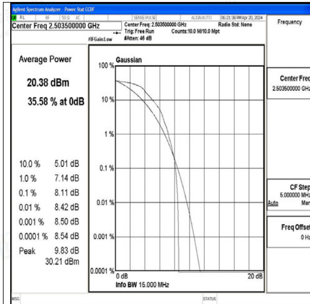
Band41-15MHz-QPSK-39725-1RB#0-PASS
