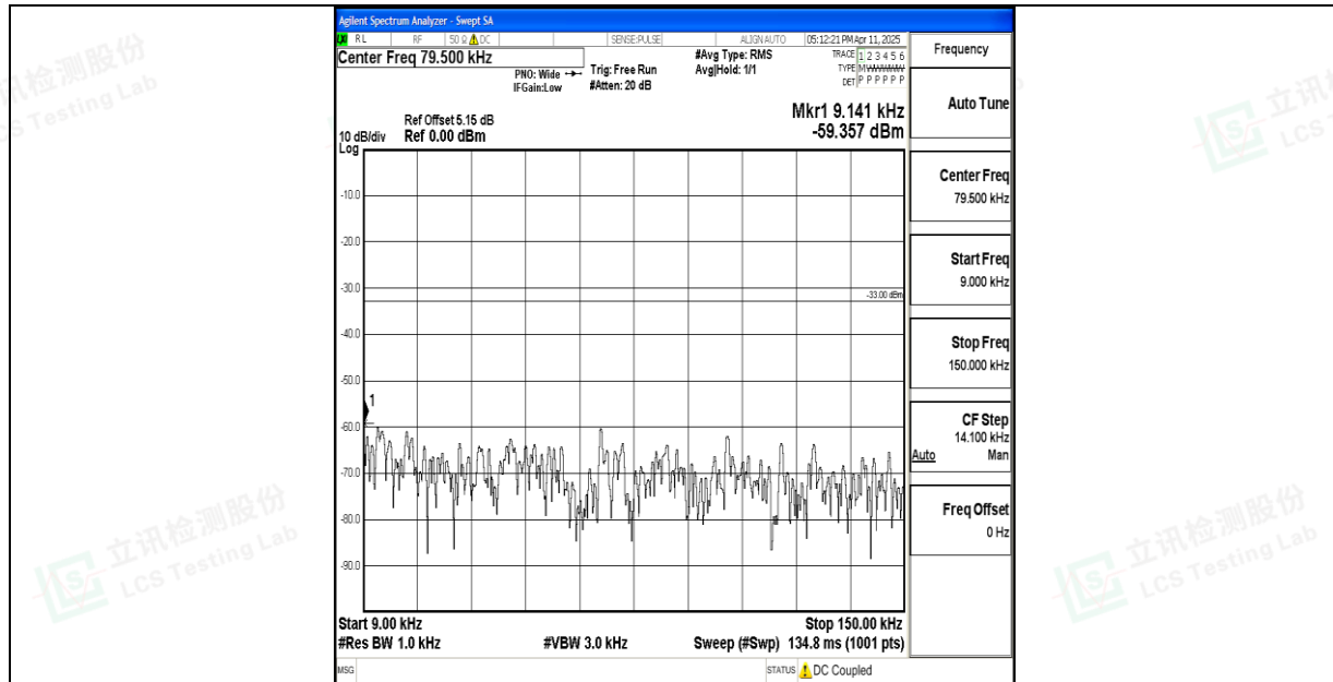
Band17_10MHz_16QAM_23790_1RB#0_0.009~0.15_0.009~0.15
