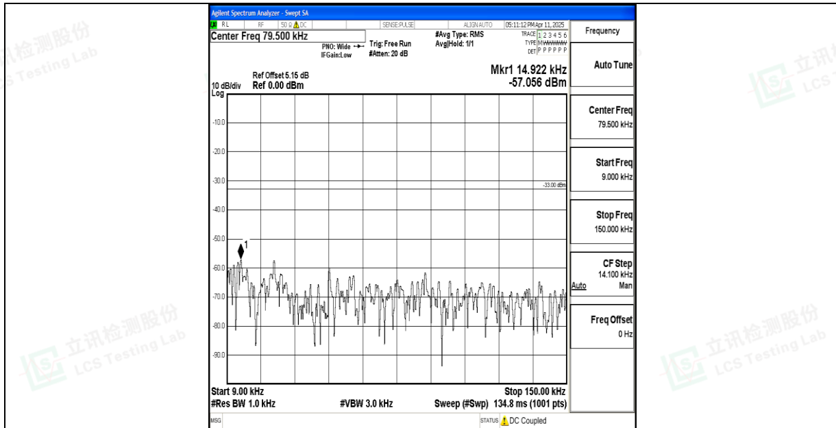
Band17_10MHz_16QAM_23780_1RB#0_0.009~0.15_0.009~0.15
