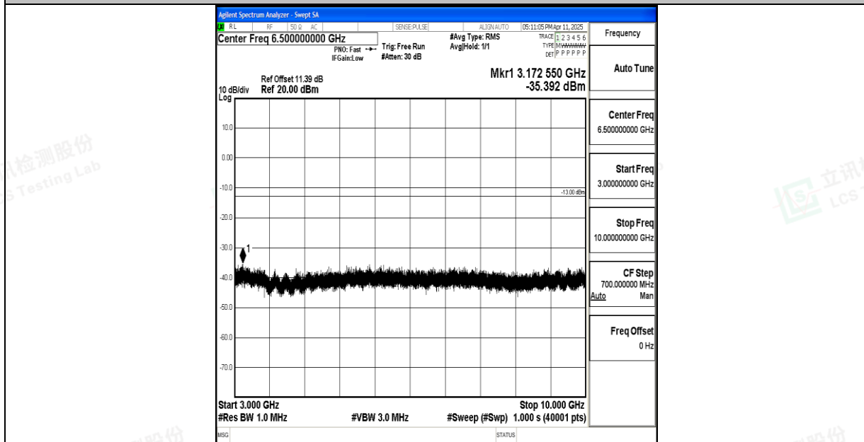
Band17_10MHz_QPSK_23780_1RB#0_3000~10000_3000~10000
