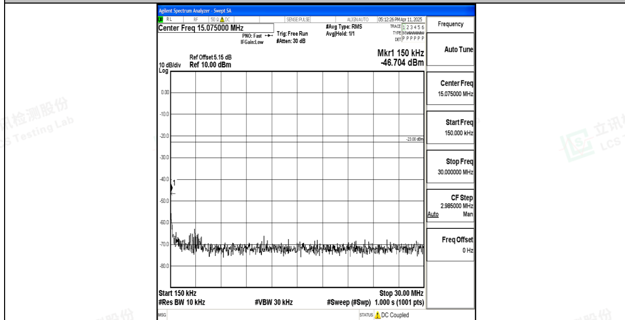
Band17_10MHz_16QAM_23790_1RB#0_0.15~30_0.15~30
