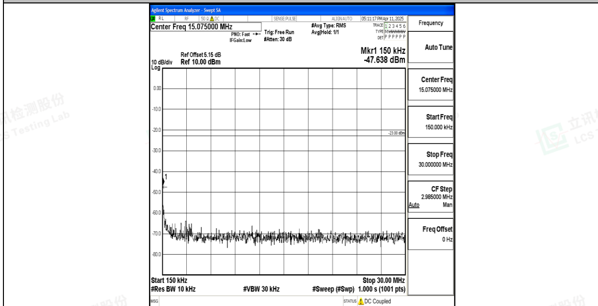
Band17_10MHz_16QAM_23780_1RB#0_0.15~30_0.15~30
