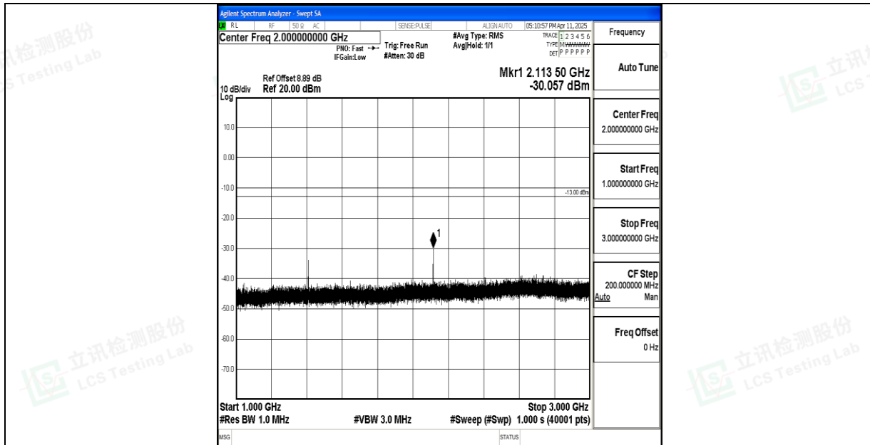
Band17_10MHz_QPSK_23780_1RB#0_1000~3000_1000~3000
