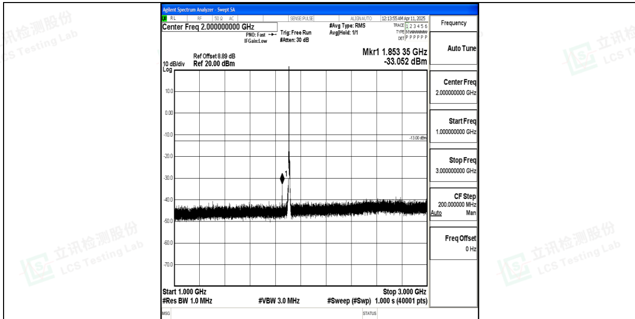
Band25_10MHz_QPSK_26640_1RB#0_1000~3000_1000~3000
