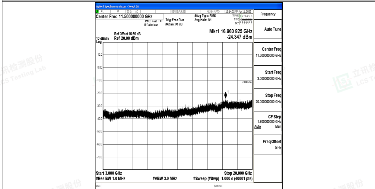
Band25_10MHz_QPSK_26640_1RB#0_3000~20000_3000~20000
