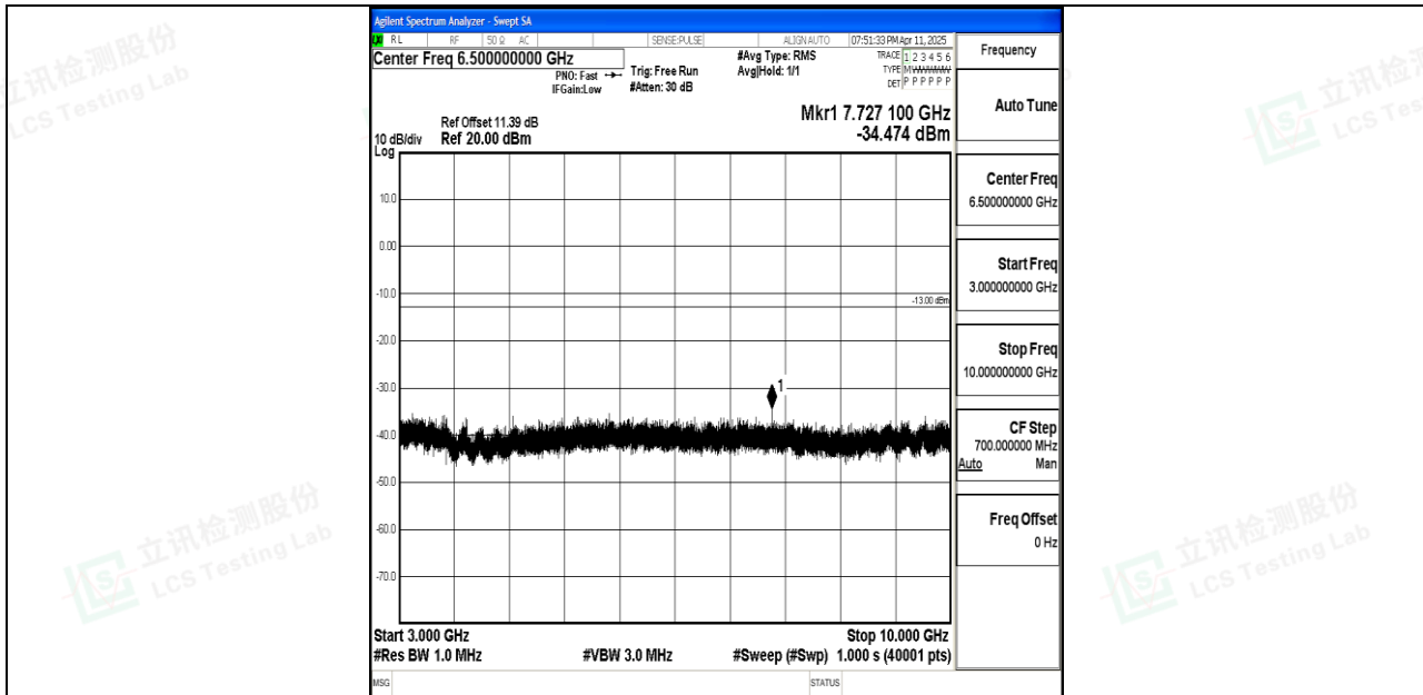
Band26_15MHz_QPSK_26965_1RB#0_3000~10000_3000~10000
