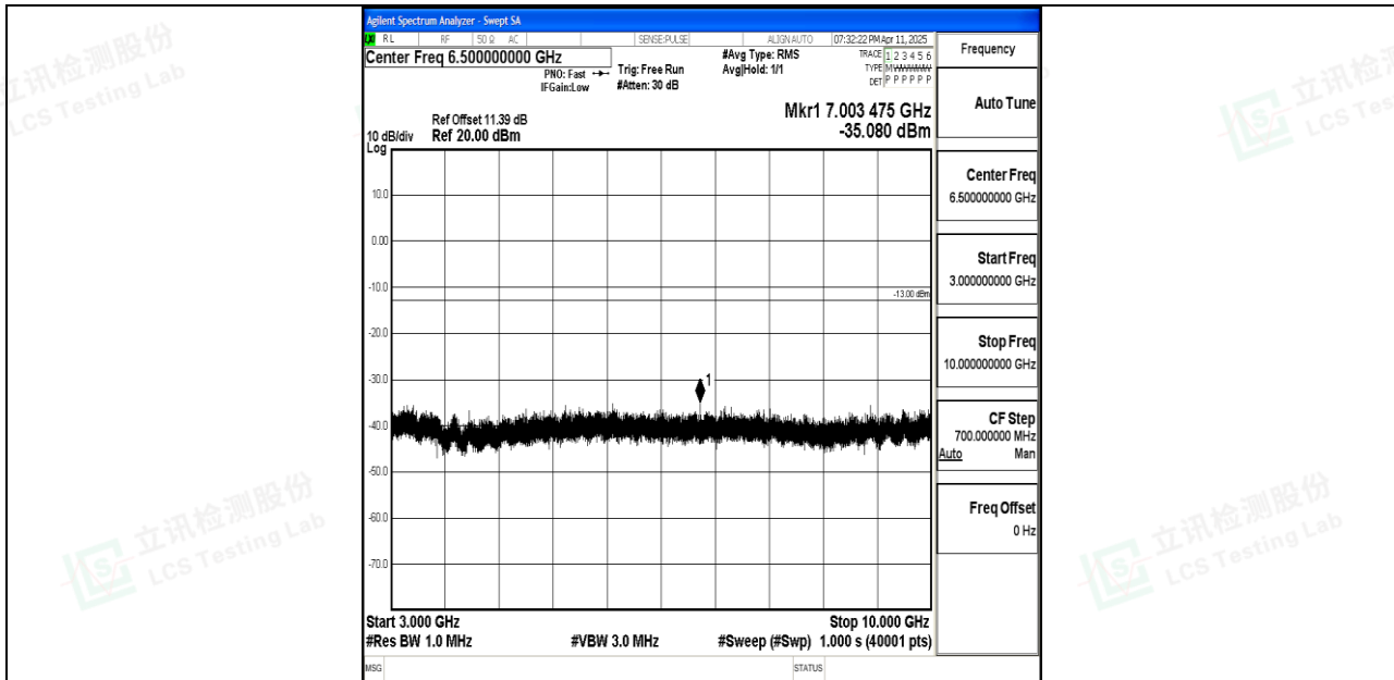
Band26_10MHz_QPSK_26840_1RB#0_3000~10000_3000~10000
