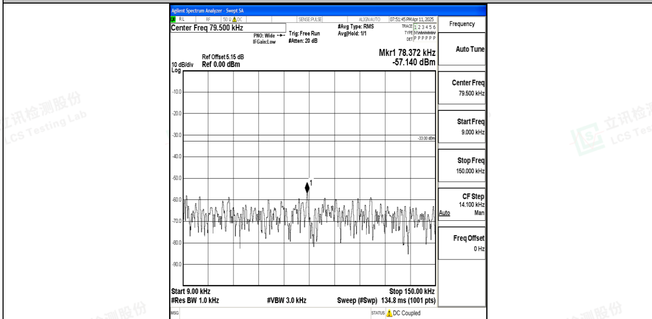
Band26_15MHz_16QAM_26965_1RB#0_0.009~0.15_0.009~0.15
