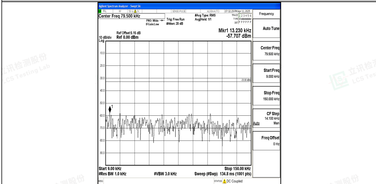
Band26_10MHz_16QAM_26840_1RB#0_0.009~0.15_0.009~0.15
