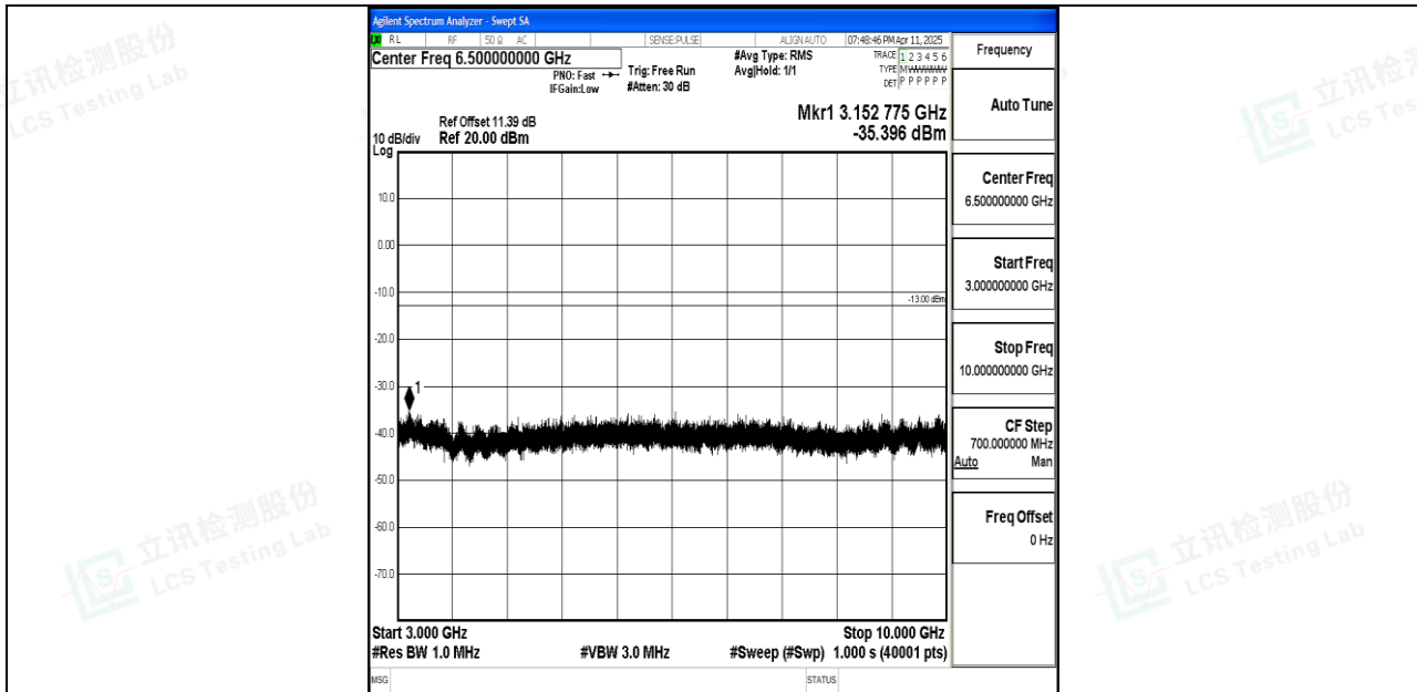
Band26_15MHz_QPSK_26865_1RB#0_3000~10000_3000~10000
