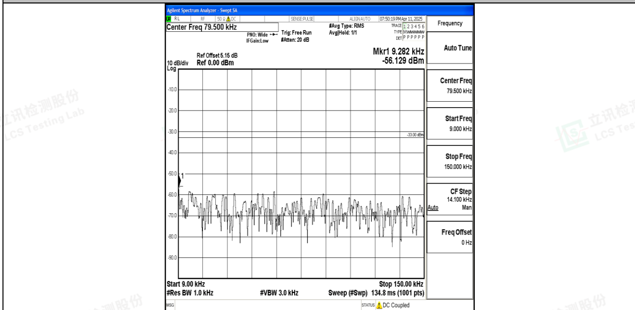
Band26_15MHz_16QAM_26915_1RB#0_0.009~0.15_0.009~0.15
