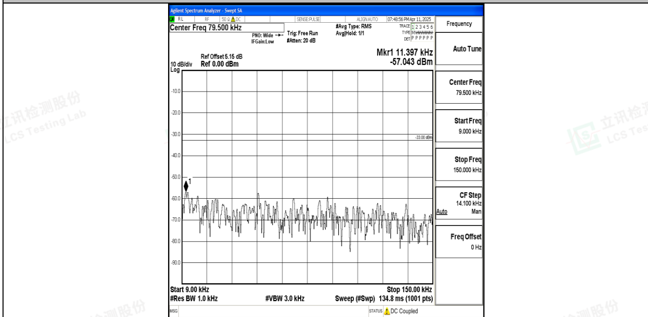
Band26_15MHz_16QAM_26865_1RB#0_0.009~0.15_0.009~0.15
