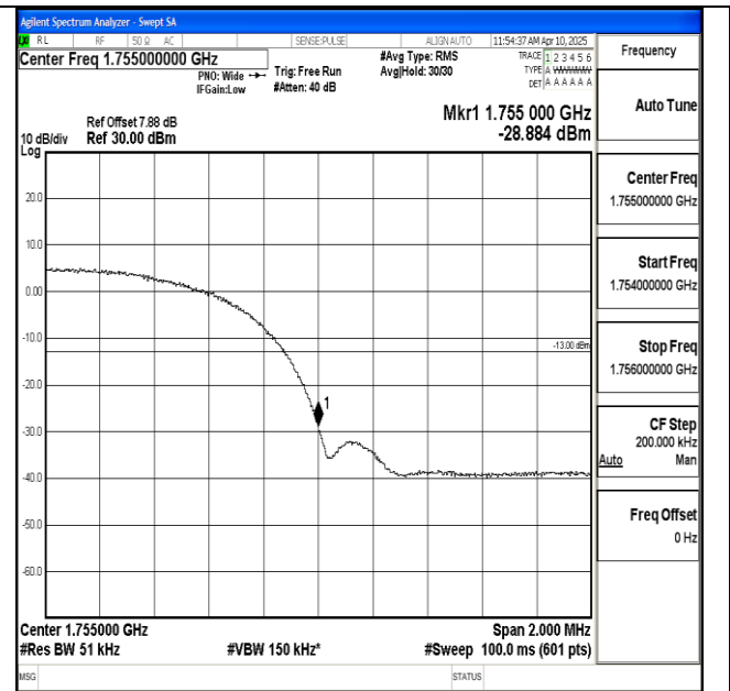
Channel 1513 / 1752.6 MHz
