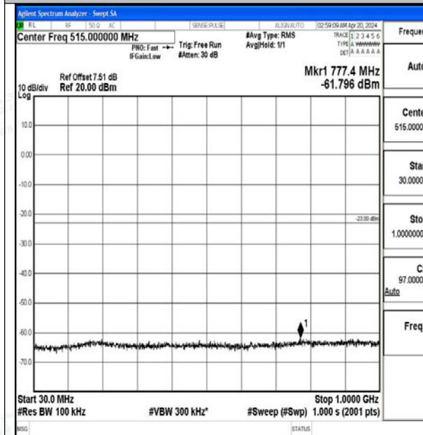
Band2_20MHz_QPSK_18900_1RB#0_30~1000_30~1000
