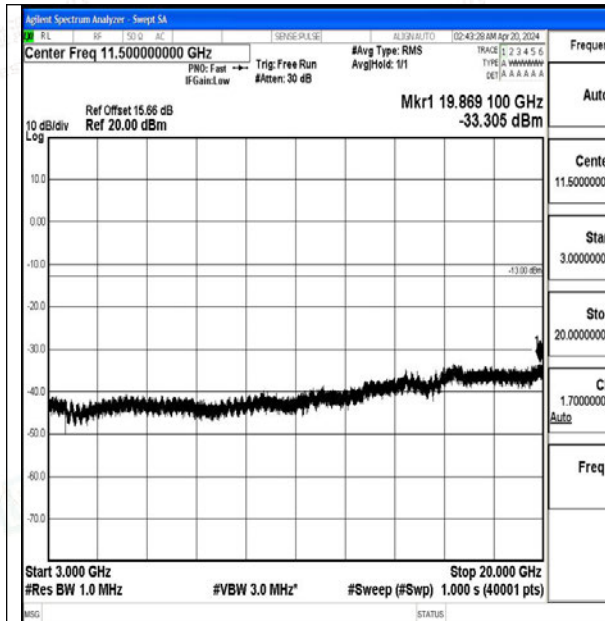
Band2_15MHz_QPSK_19125_1RB#0_3000~20000_3000~20000
