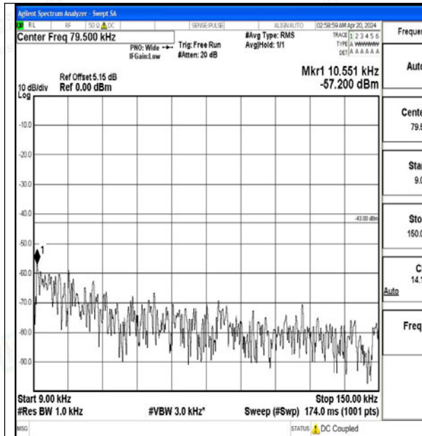
Band2_20MHz_QPSK_18900_1RB#0_0.009~0.15_0.009~0.15
