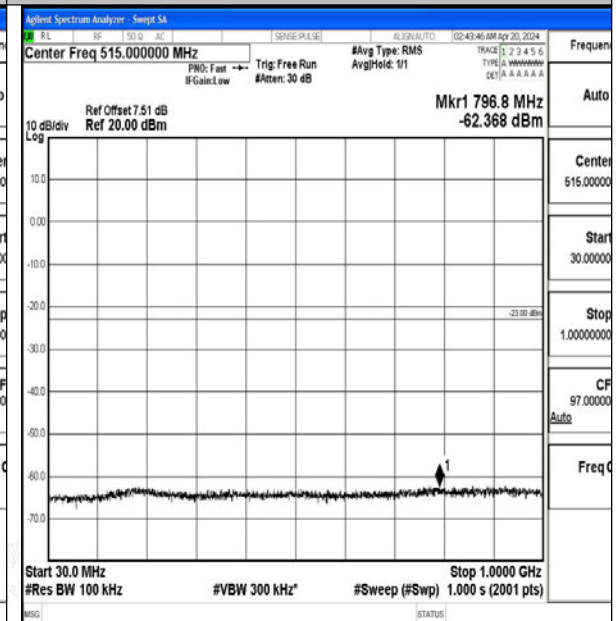
Band2_15MHz_16QAM_19125_1RB#0_30~1000_30~1000
