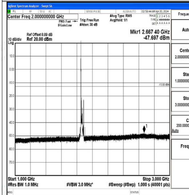
Band2_20MHz_16QAM_18700_1RB#0_1000~3000_ 1000~3000
