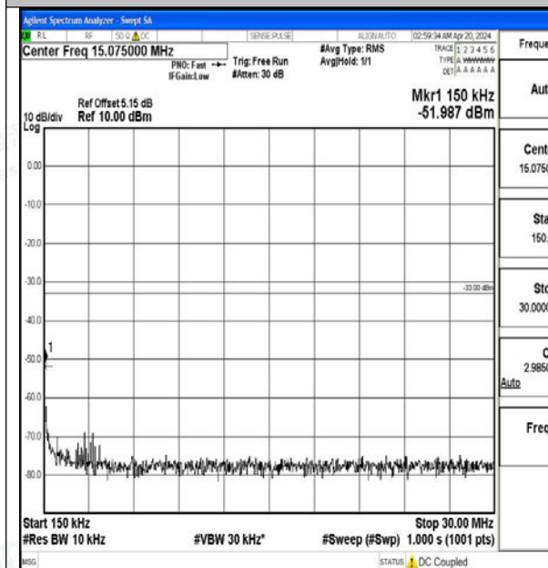
Band2_20MHz_16QAM_18900_1RB#0_0.15~30_0.15~30
