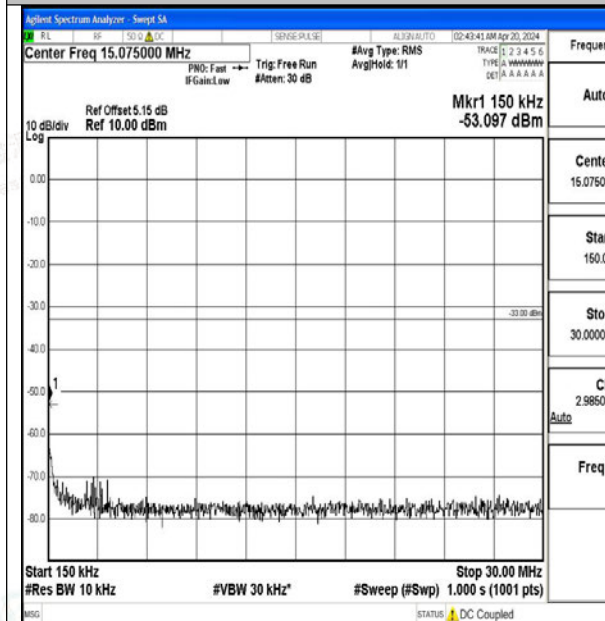
Band2_15MHz_16QAM_19125_1RB#0_0.15~30_0.15~30
