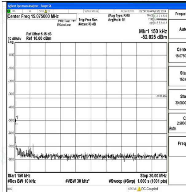
Band2_20MHz_16QAM_18700_1RB#0_0.15~30_0.1 5~30
