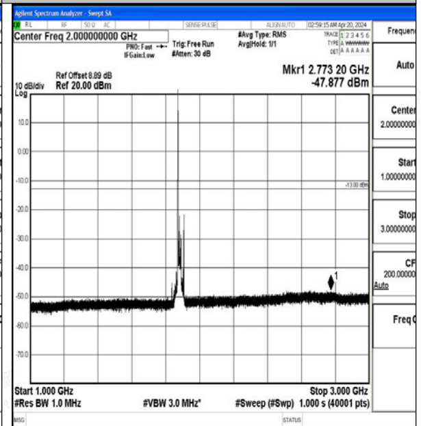
Band2_20MHz_QPSK_18900_1RB#0_1000~3000_1000~3000
