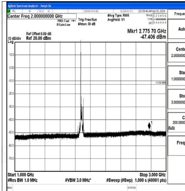
Band2_20MHz_16QAM_18900_1RB#0_1000~3000_1000~3000
