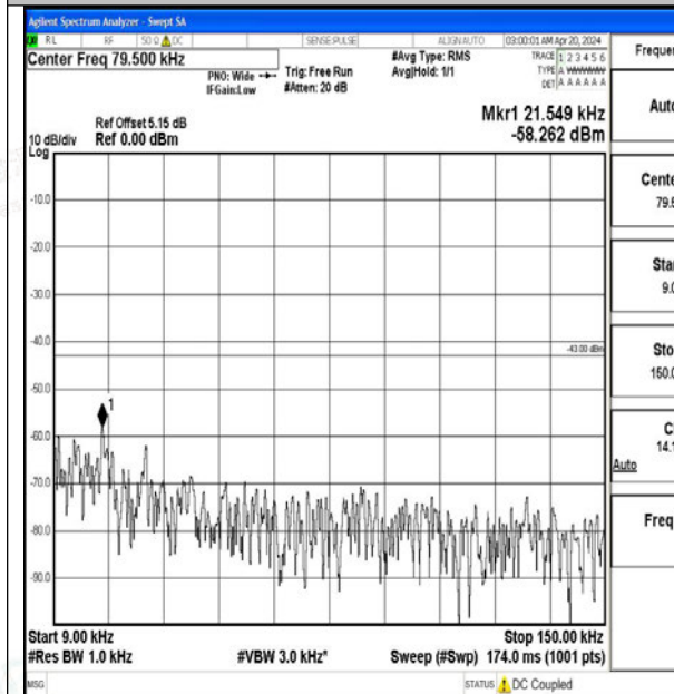
Band2_20MHz_QPSK_19100_1RB#0_0.009~0.15_0.009~0.15
