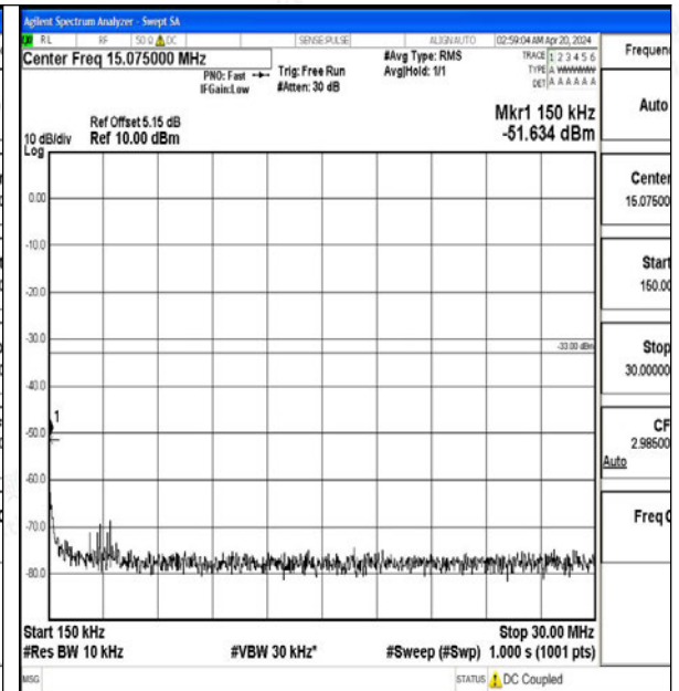
Band2_20MHz_QPSK_18900_1RB#0_0.15~30_0.15~30
