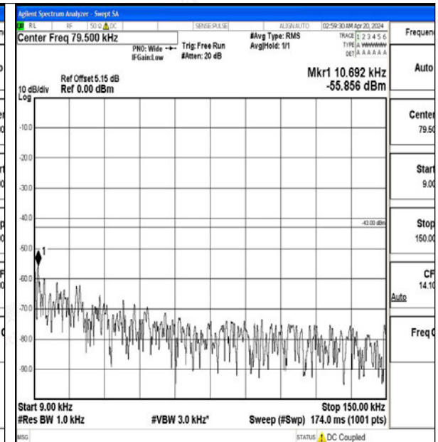
Band2_20MHz_16QAM_18900_1RB#0_0.009~0.15_0.009~0.15
