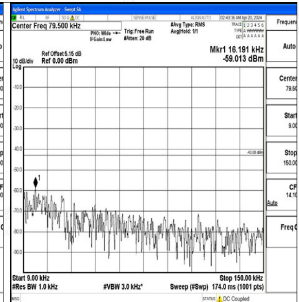
Band2_15MHz_16QAM_19125_1RB#0_0.009~0.15_0.009~0.15
