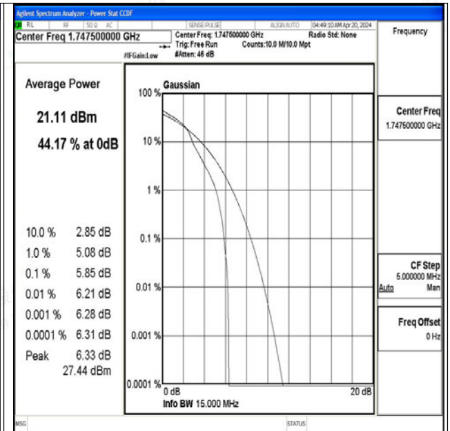
Band4-15MHz-16QAM-20325-1RB#0-PASS
