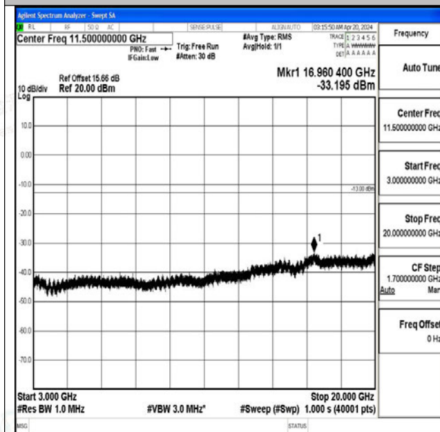
Band4_1.4MHz_QPSK_20175_1RB#0_3000~20000_3000
