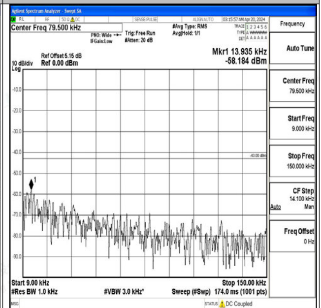
Band4_1.4MHz_16QAM_20175_1RB#0_0.009~0.15_0.0
