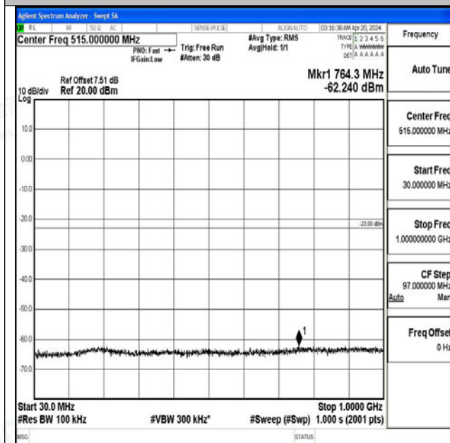
Band4_1.4MHz_QPSK_20393_1RB#0_30~1000_30~100 0
