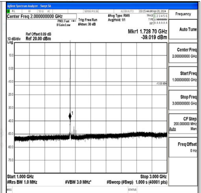
Band4_1.4MHz_QPSK_20175_1RB#0_1000~3000_1000
